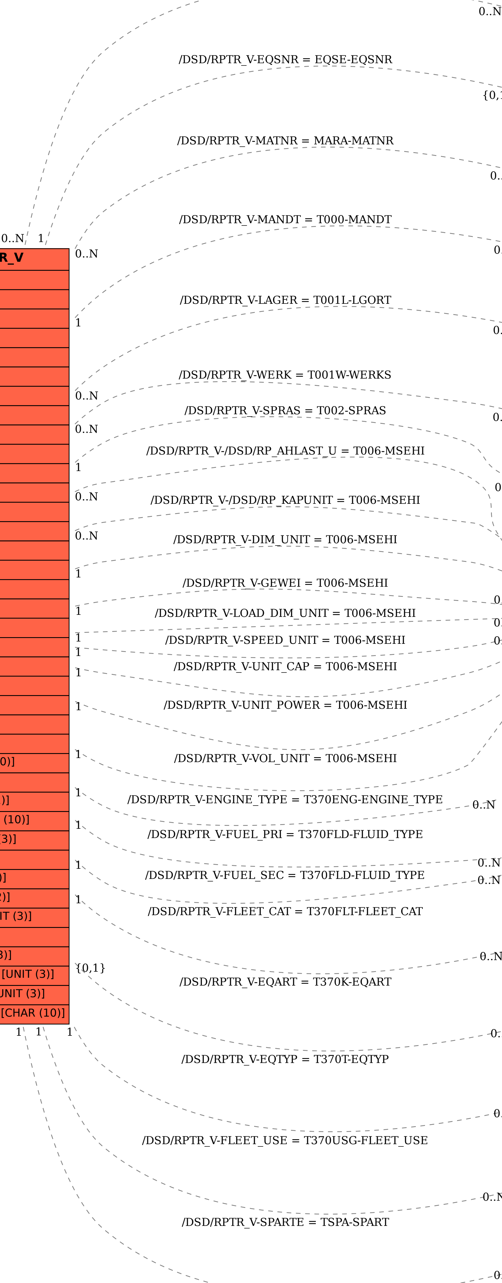
SAP ABAP table /DSD/RPTR_V {Generated Table for View} /DSD/RPTR_V-VSO/M_VSO_FTYPE = /VSO/B_FLEET-VSO_FTYPE
