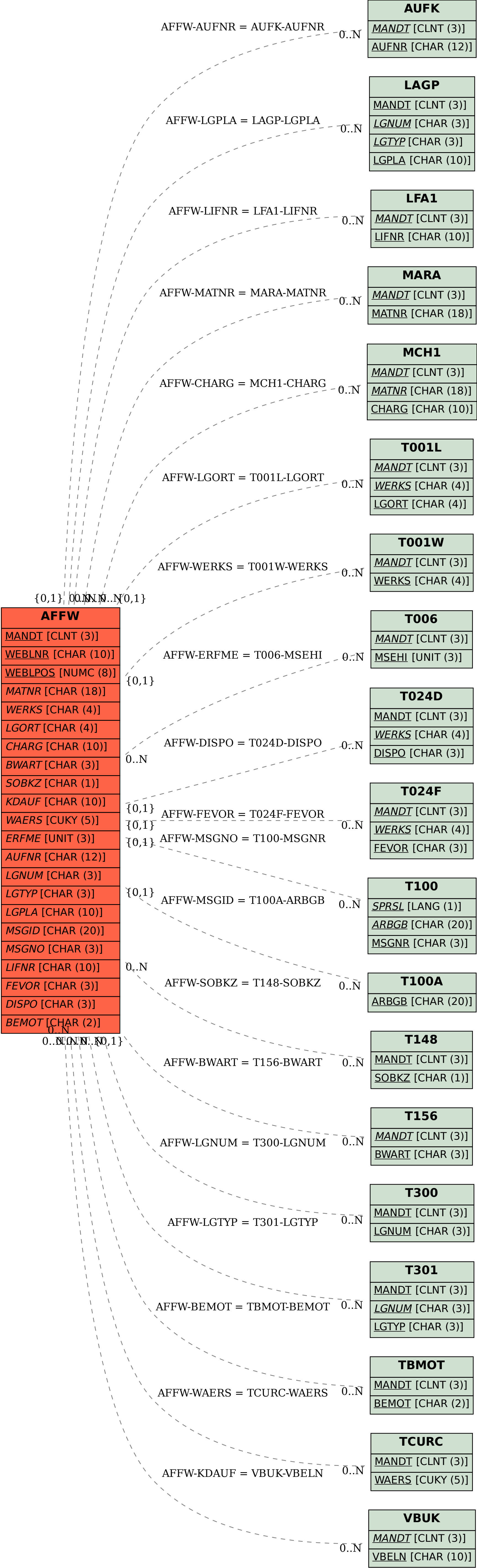
SAP ABAP table AFFW {Goods Movements with Errors from Confirmations}
