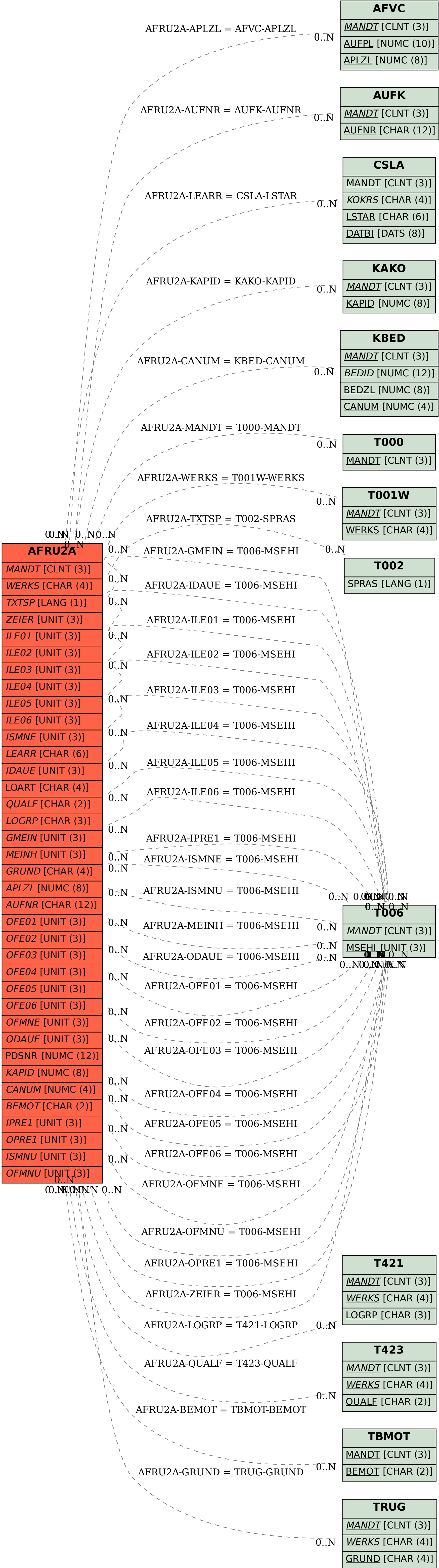
SAP ABAP table AFRU2A {Order confirmations for elements (LDB) - 02}
