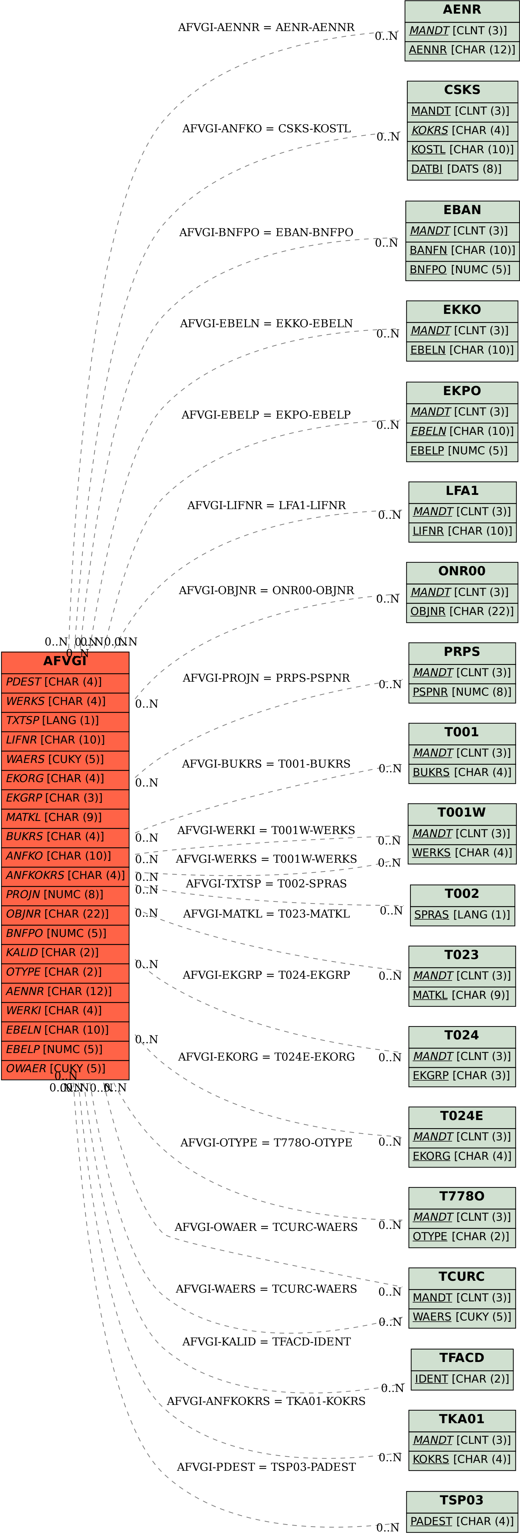
SAP ABAP table AFVGI {General include structure of the operation data}
