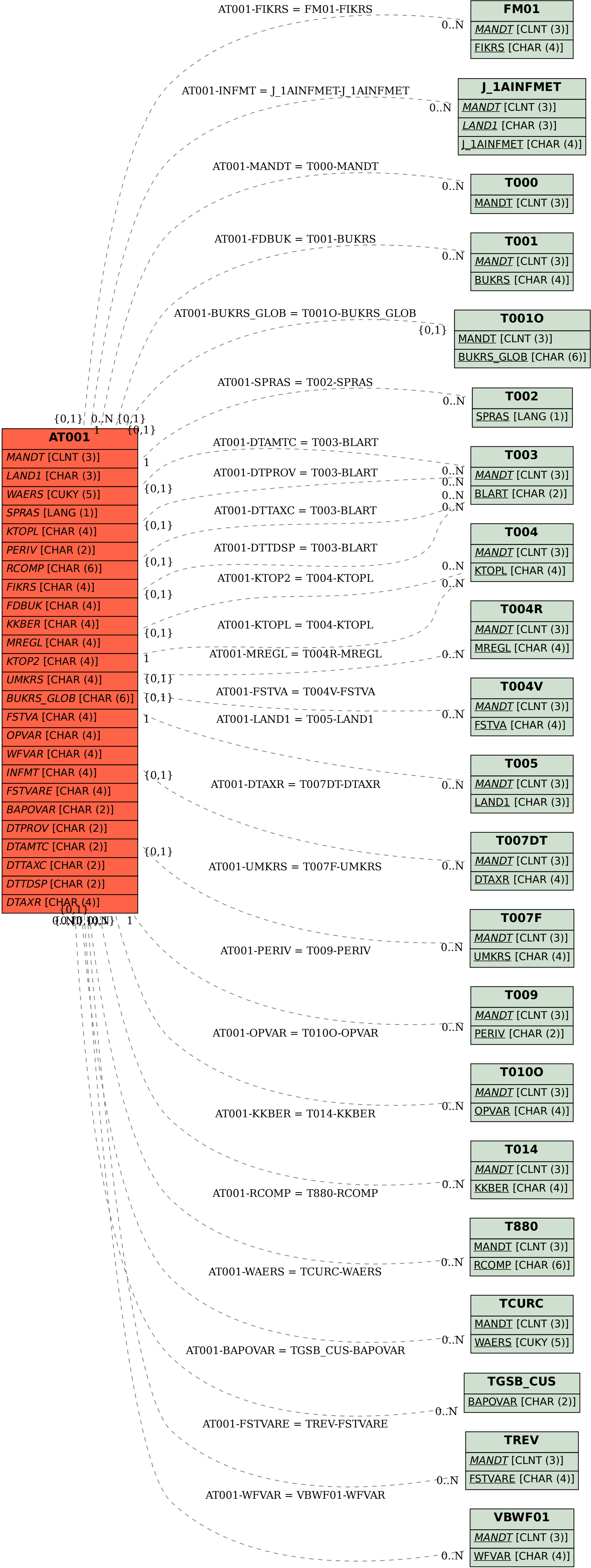
SAP ABAP table AT001 {Change Document Structure for Company Code (T001)}
