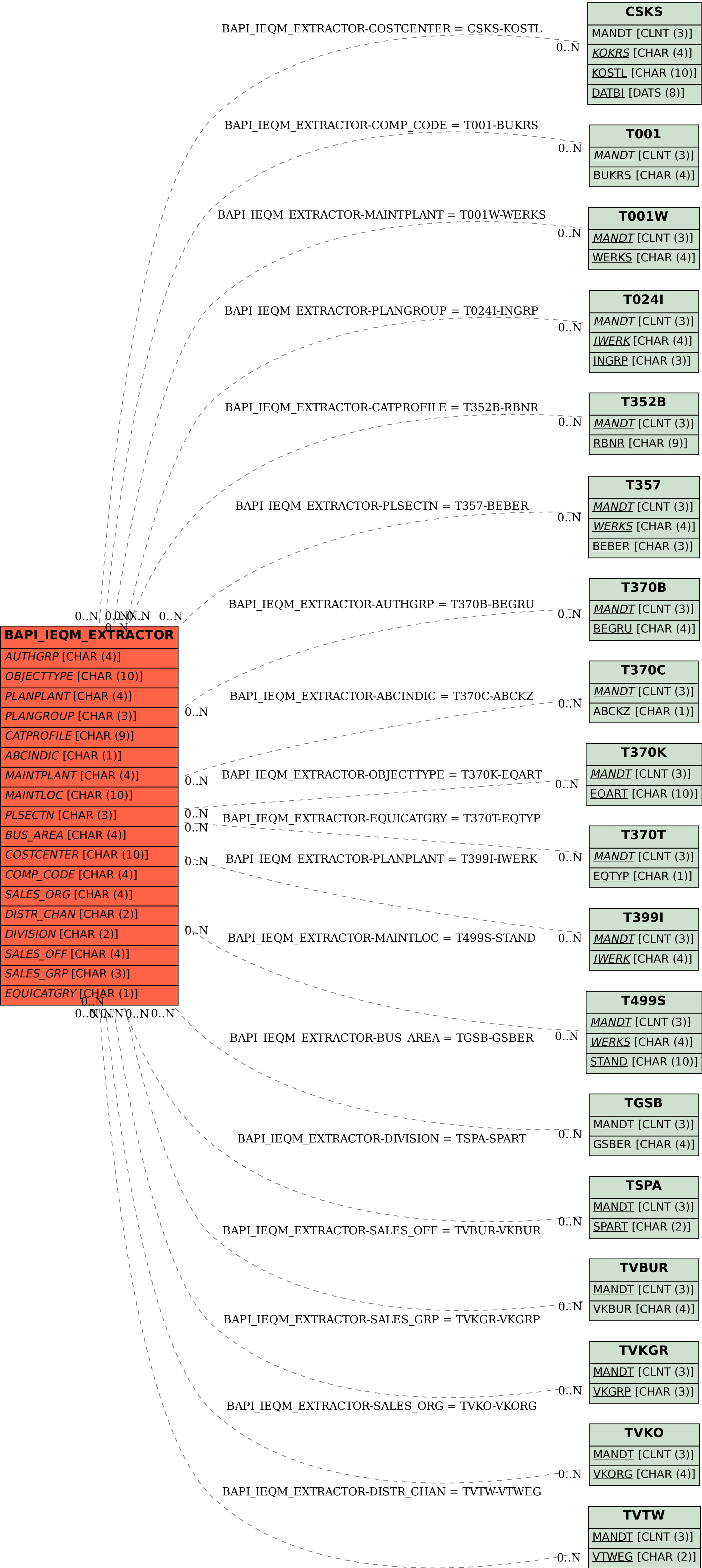
SAP ABAP table BAPI_IEQM_EXTRACTOR {BAPI Structure Data for Equipment}
