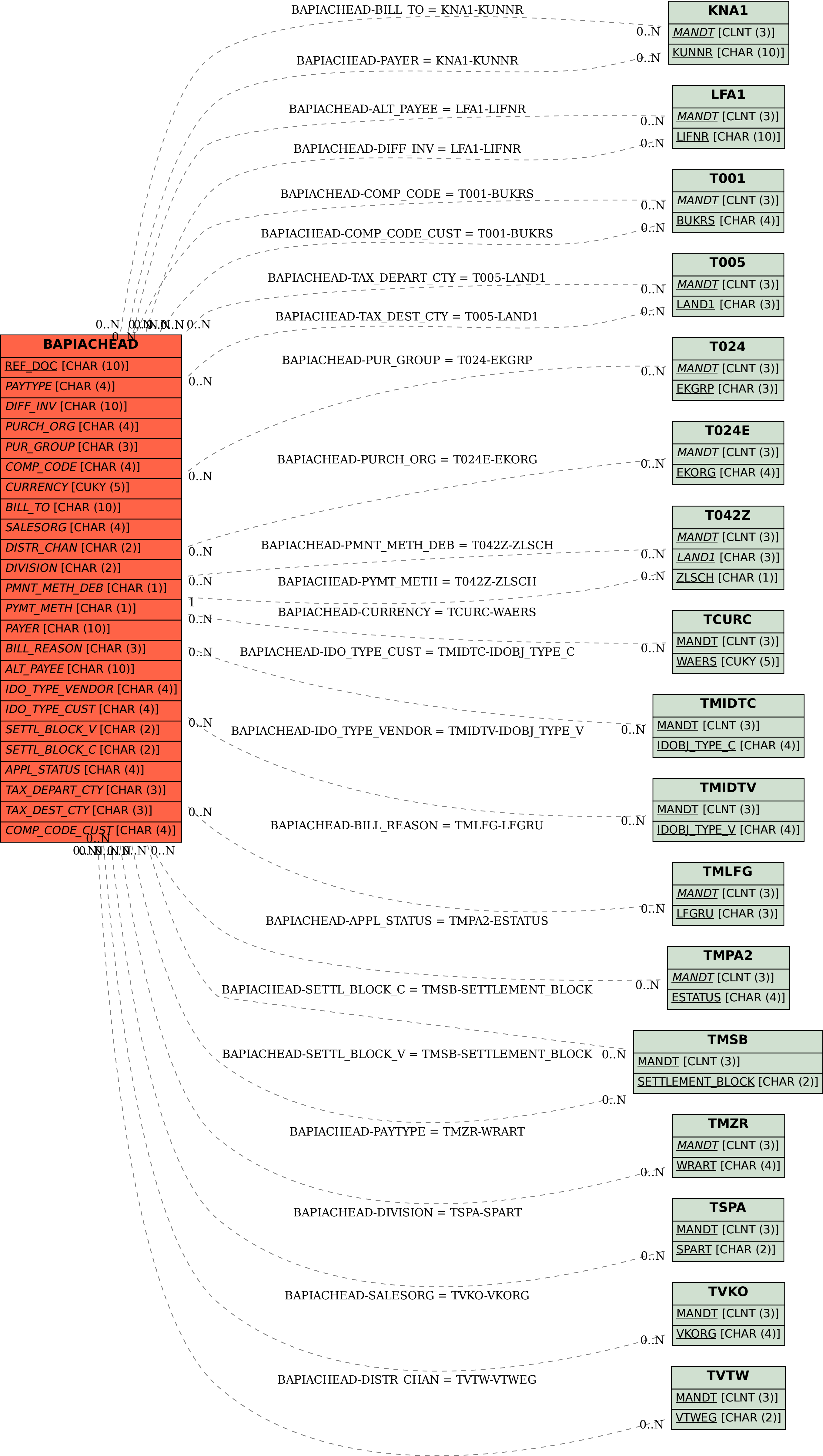
SAP ABAP table BAPIACHEAD {Communication structure: Payment document header data}
