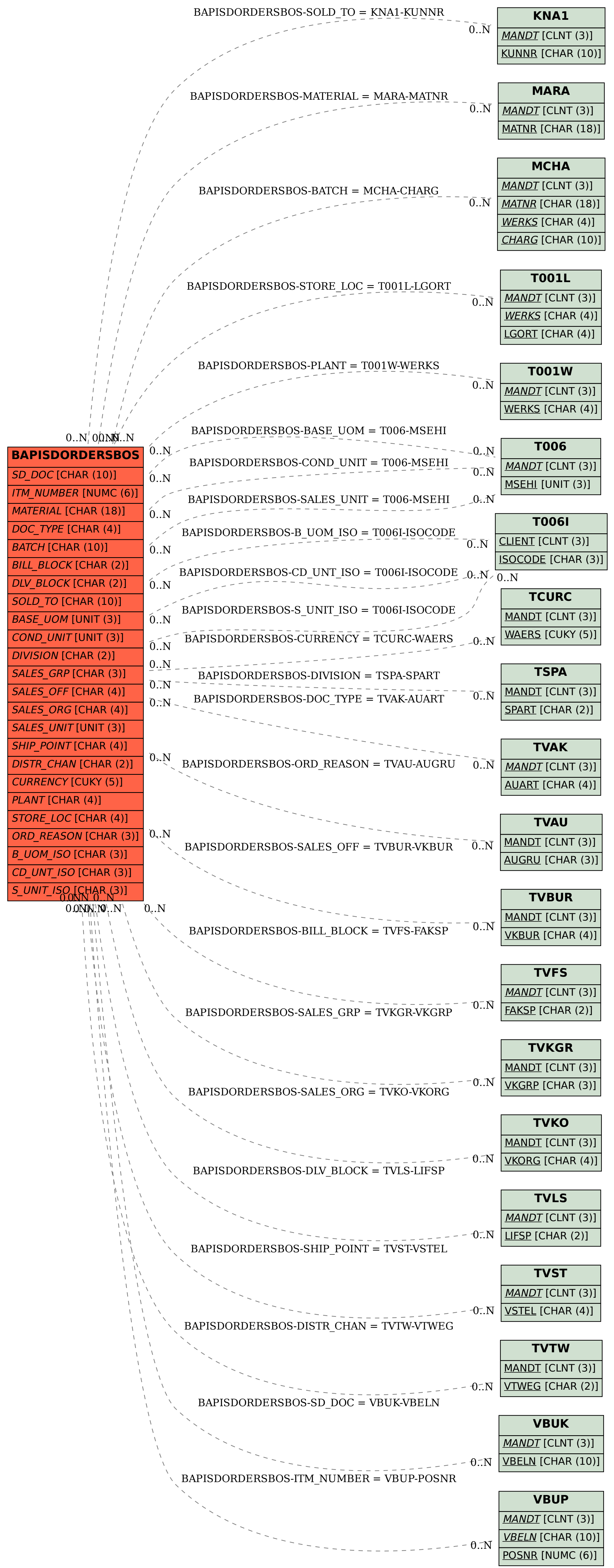
SAP ABAP table BAPISDORDERSBOS {View: Order Items (with BOS) for Material}
