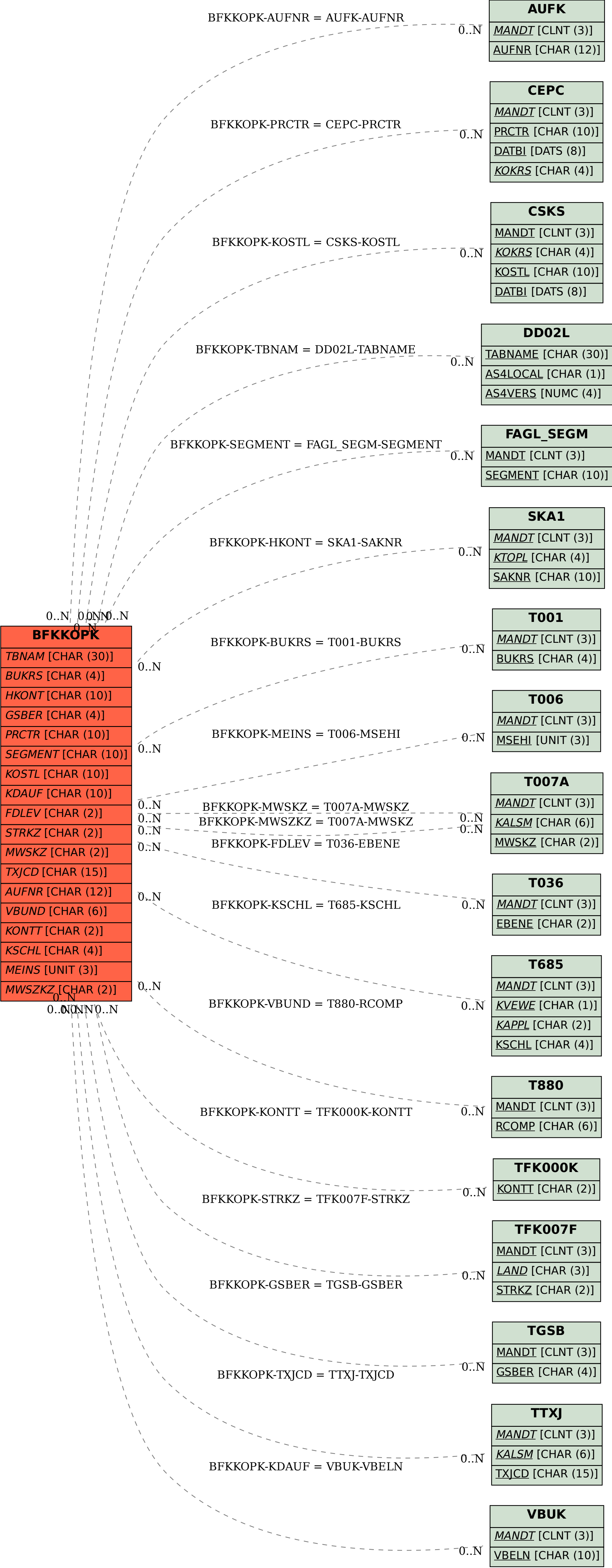
SAP ABAP table BFKKOPK {Items for accts rec/pay doc (batch input)}
