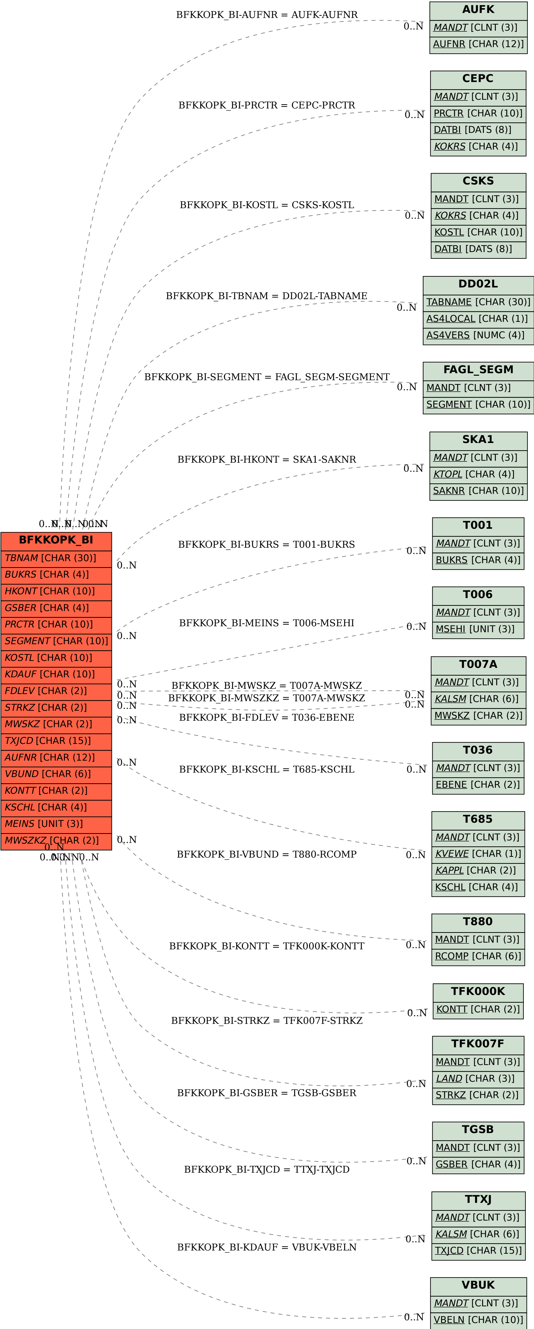
SAP ABAP table BFKKOPK_BI {Structure for events in document transfer program}
