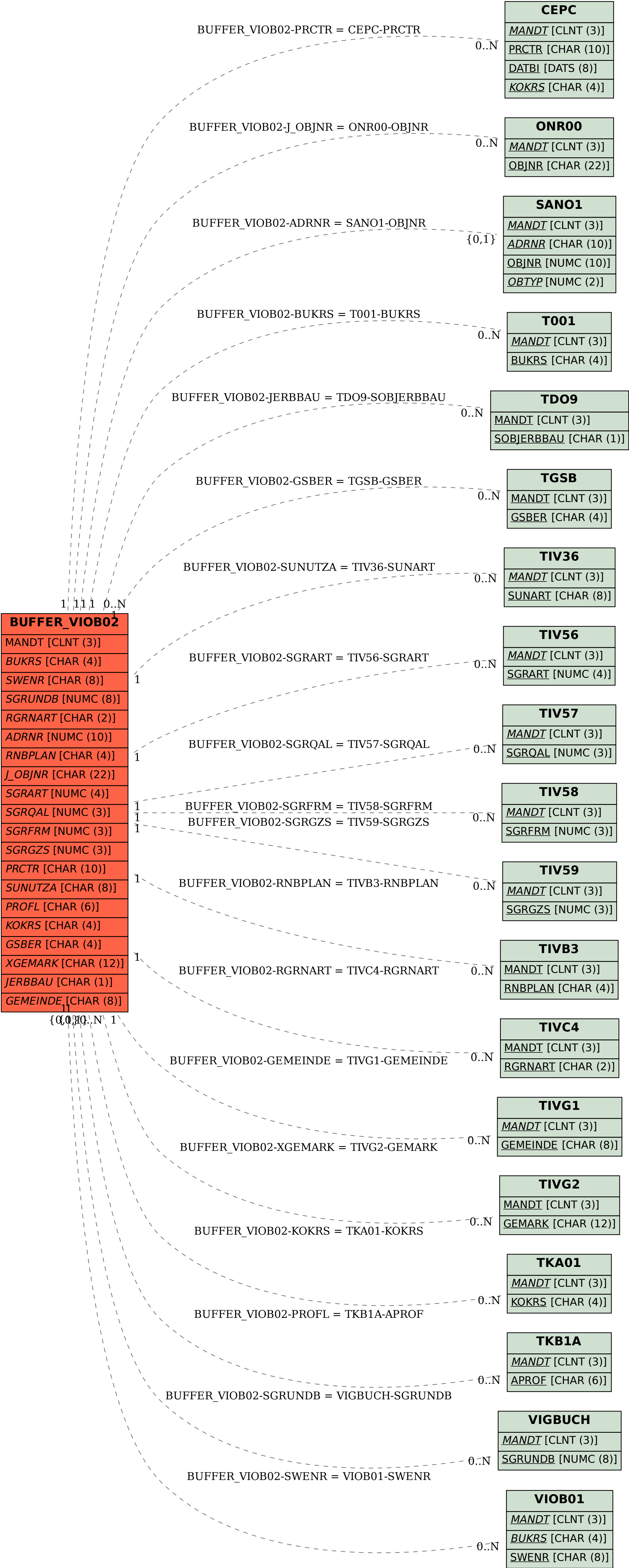
SAP ABAP table BUFFER_VIOB02 {Structure for Table Buffer for DB Table VIOB02}
