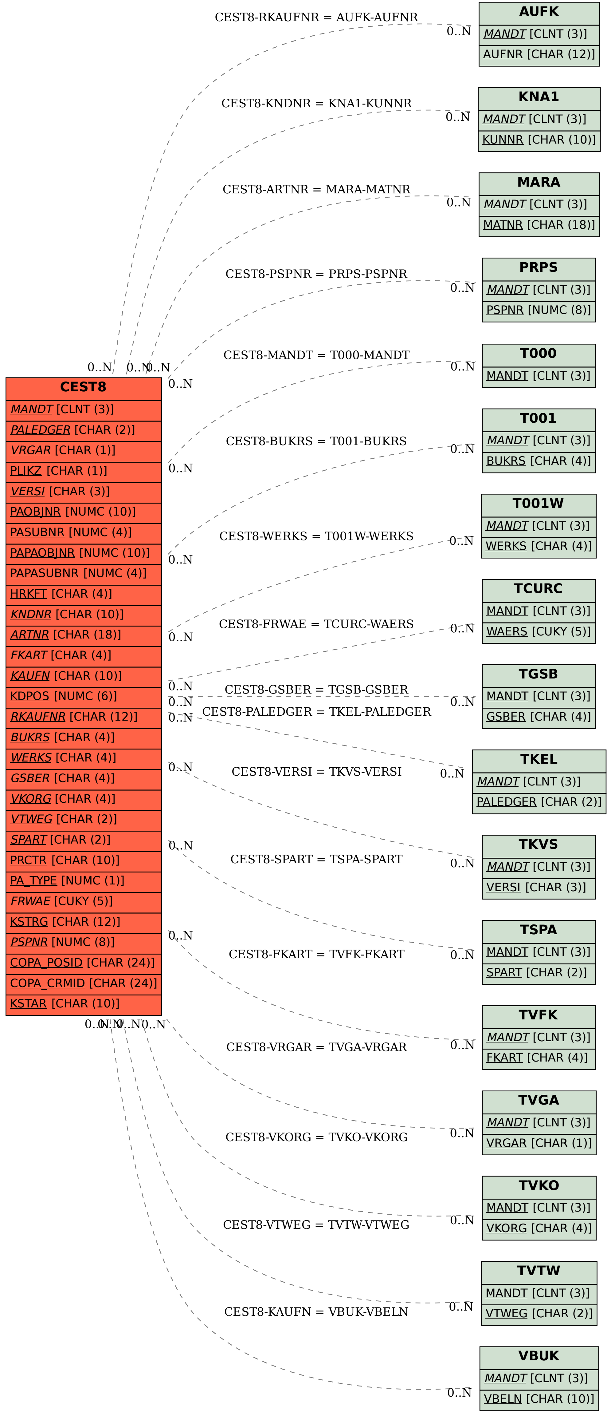
SAP ABAP table CEST8 {Transfer of cst ctr csts : Transfer str. for values}
