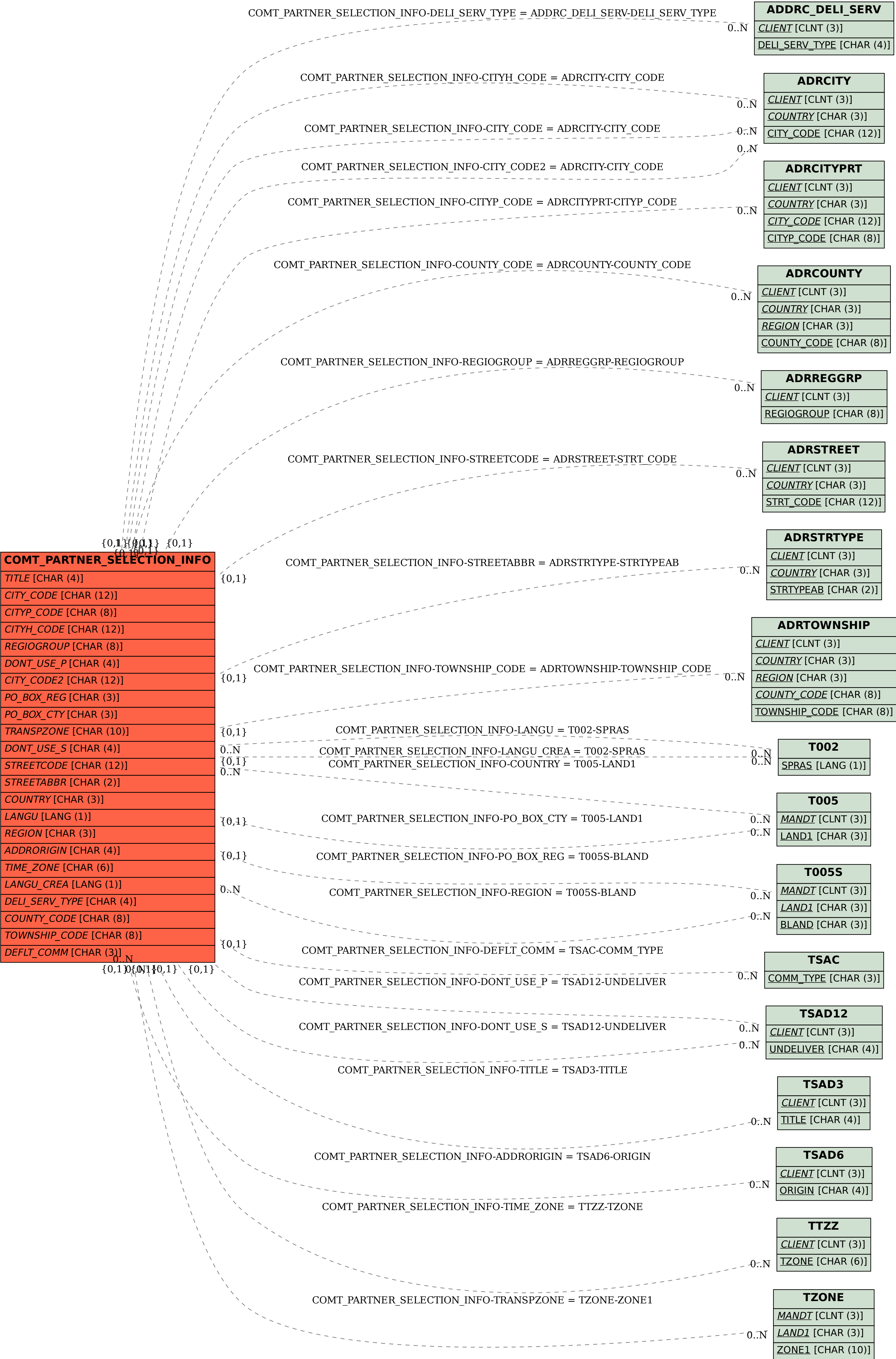
SAP ABAP table COMT_PARTNER_SELECTION_INFO {Information Structure for Partner Selection}
