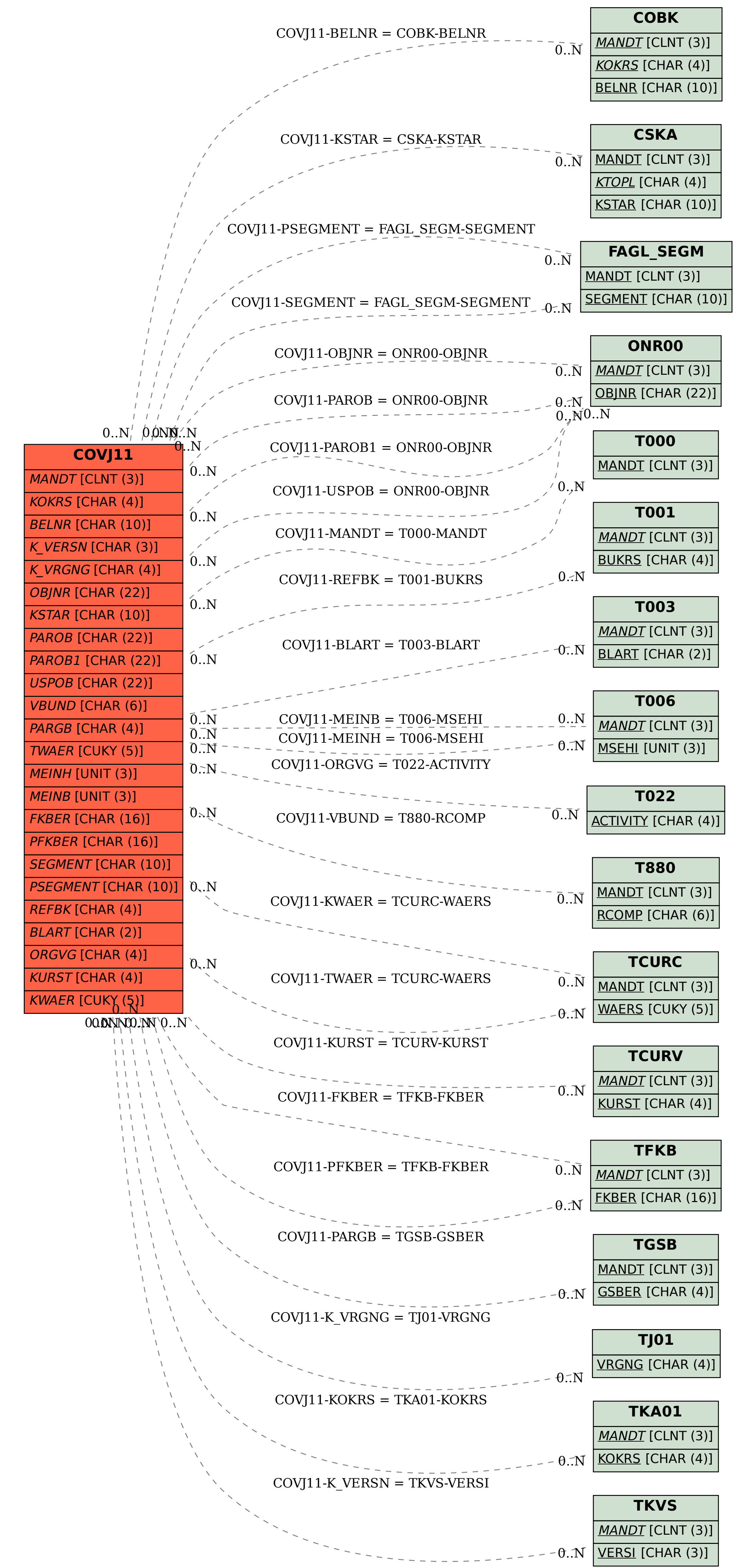
SAP ABAP table COVJ11 {CO Object: Line Items (by Year and Document Header)}
