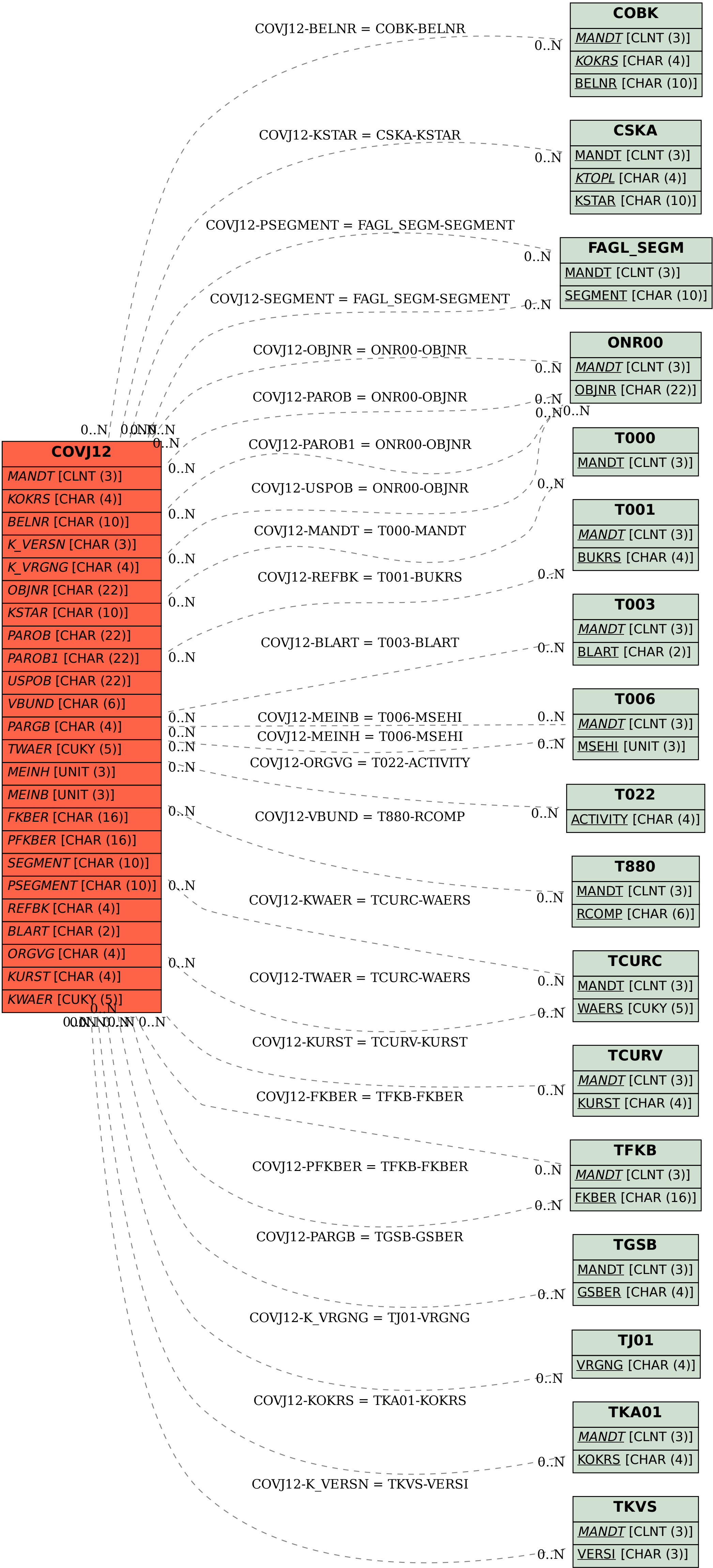
SAP ABAP table COVJ12 {CO Object: Line Items (by Year and Document Header)}
