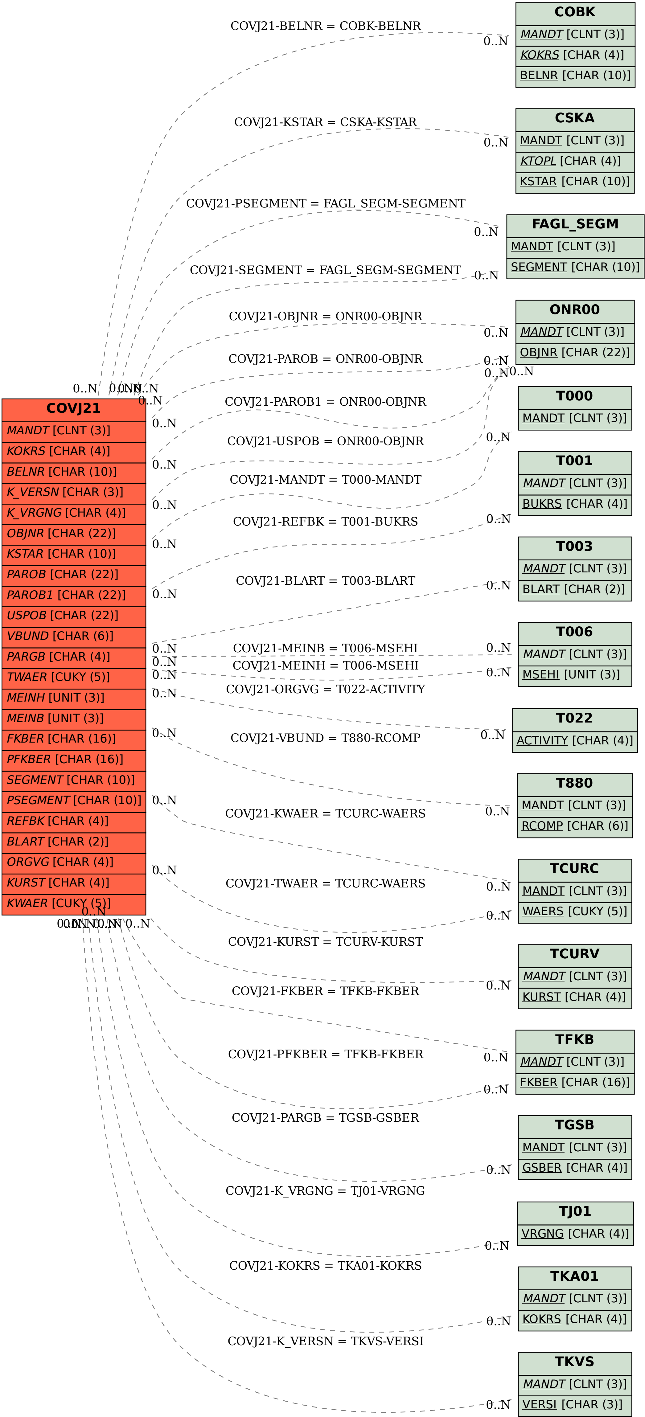
SAP ABAP table COVJ21 {CO Object: Line Items (by Year and Document Header)}
