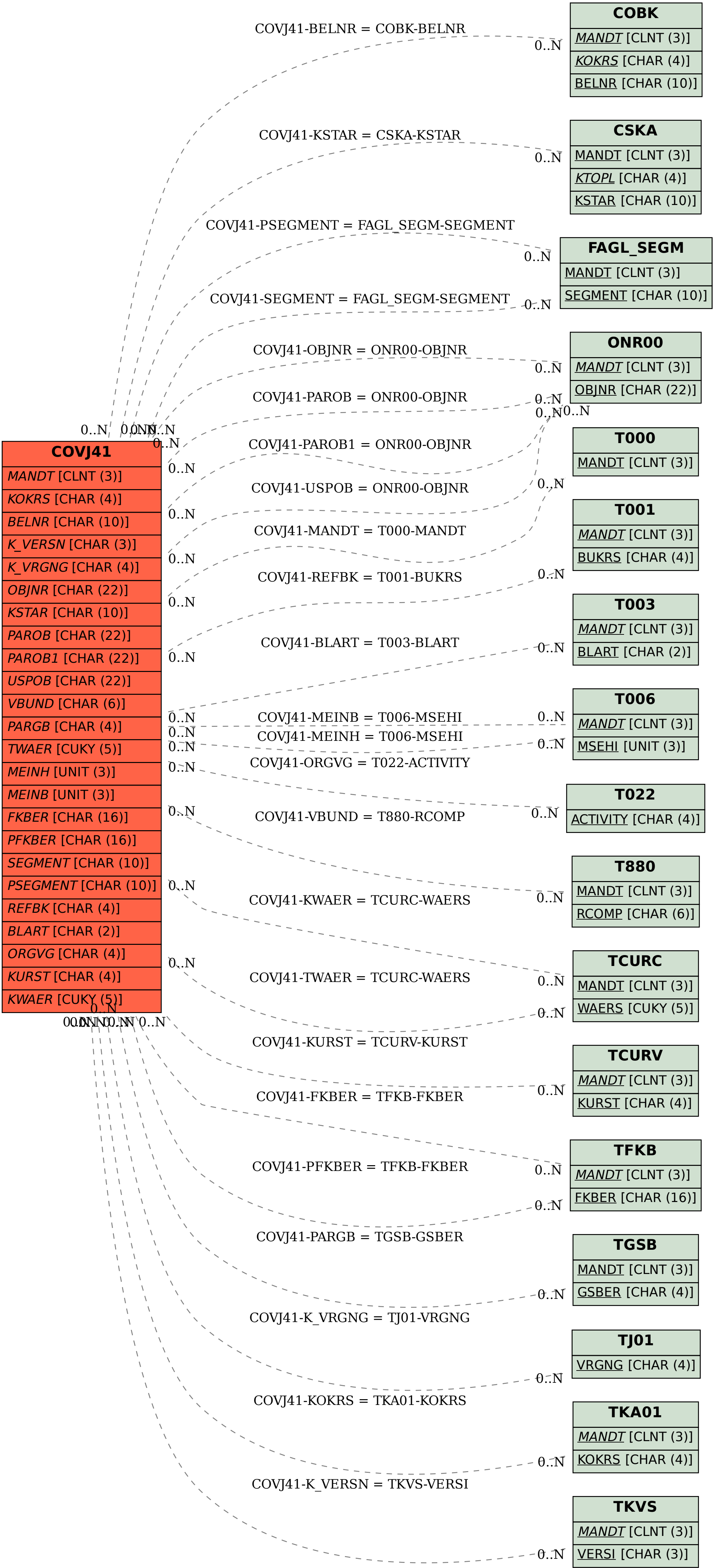
SAP ABAP table COVJ41 {CO Object: Line Items (by Year and Document Header)}
