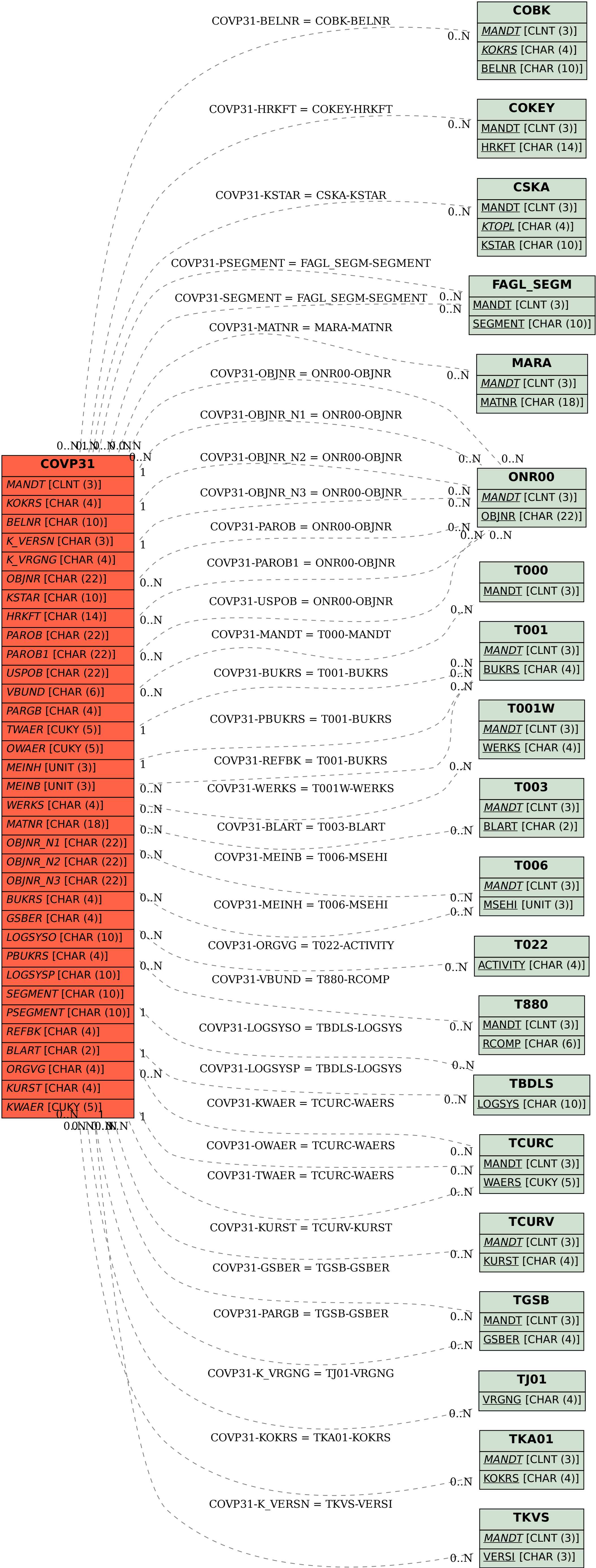
SAP ABAP table COVP31 {CO Object: Line Items (by Period and Document Header)}
