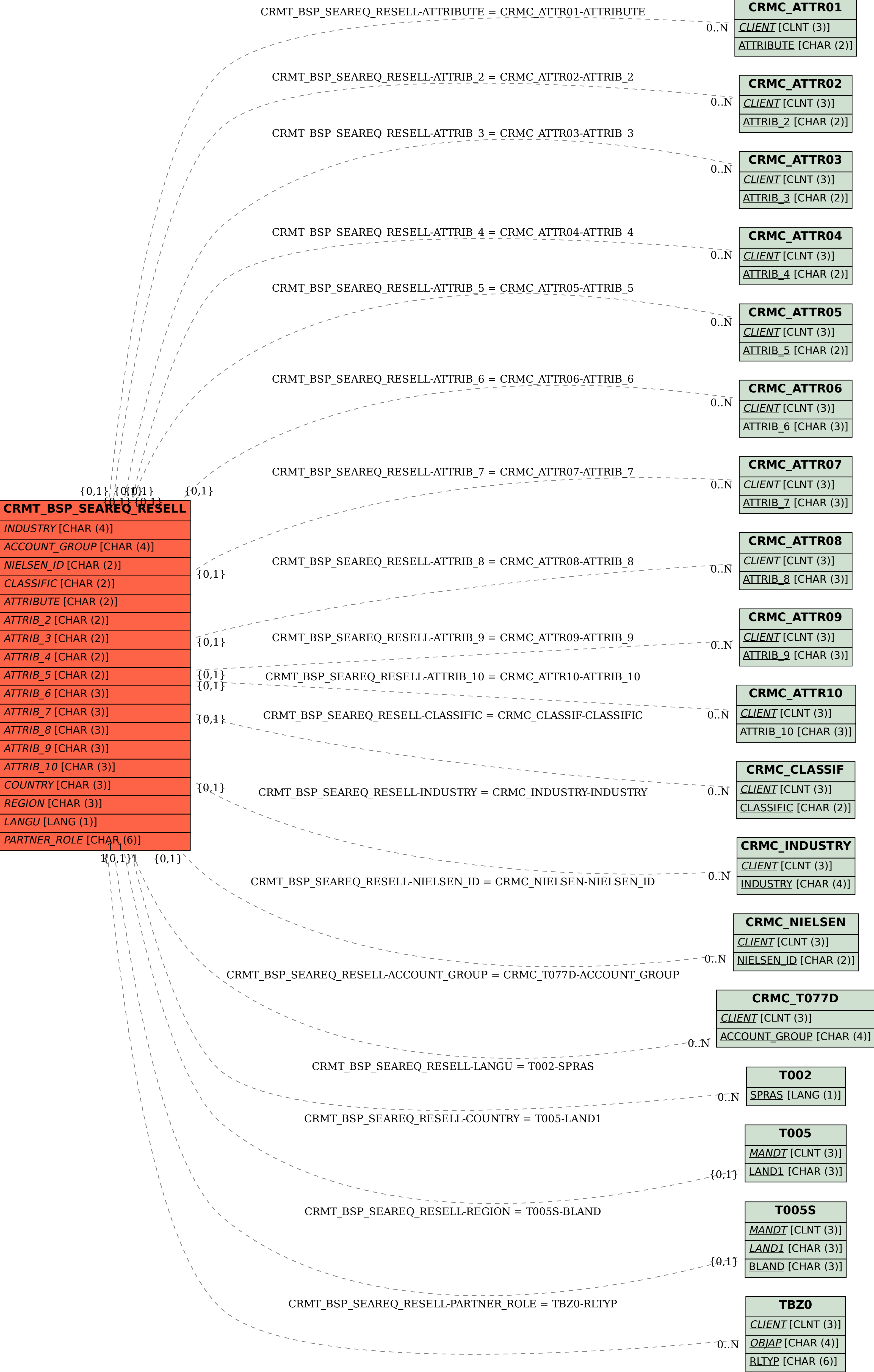
SAP ABAP table CRMT_BSP_SEAREQ_RESELL {Partner: Screen structure for OIC (End customer list)}
