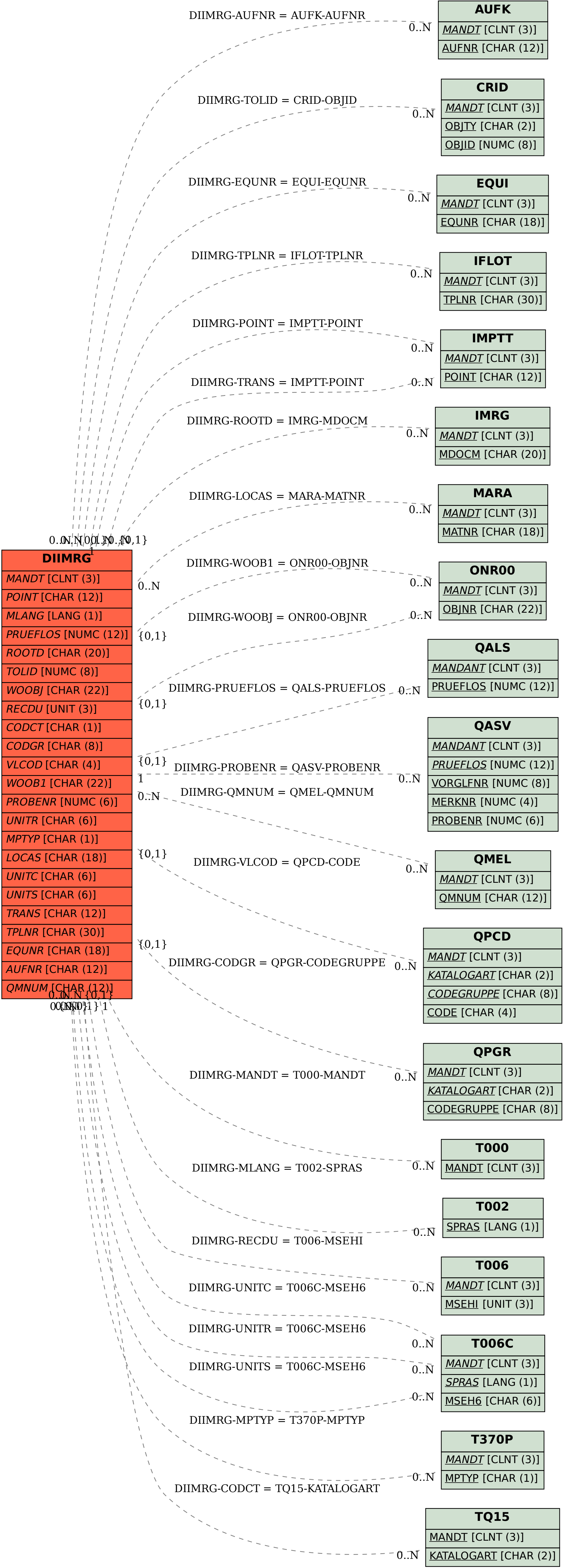
SAP ABAP table DIIMRG {Measurement Document: Output Structure for ABAP Lists}
