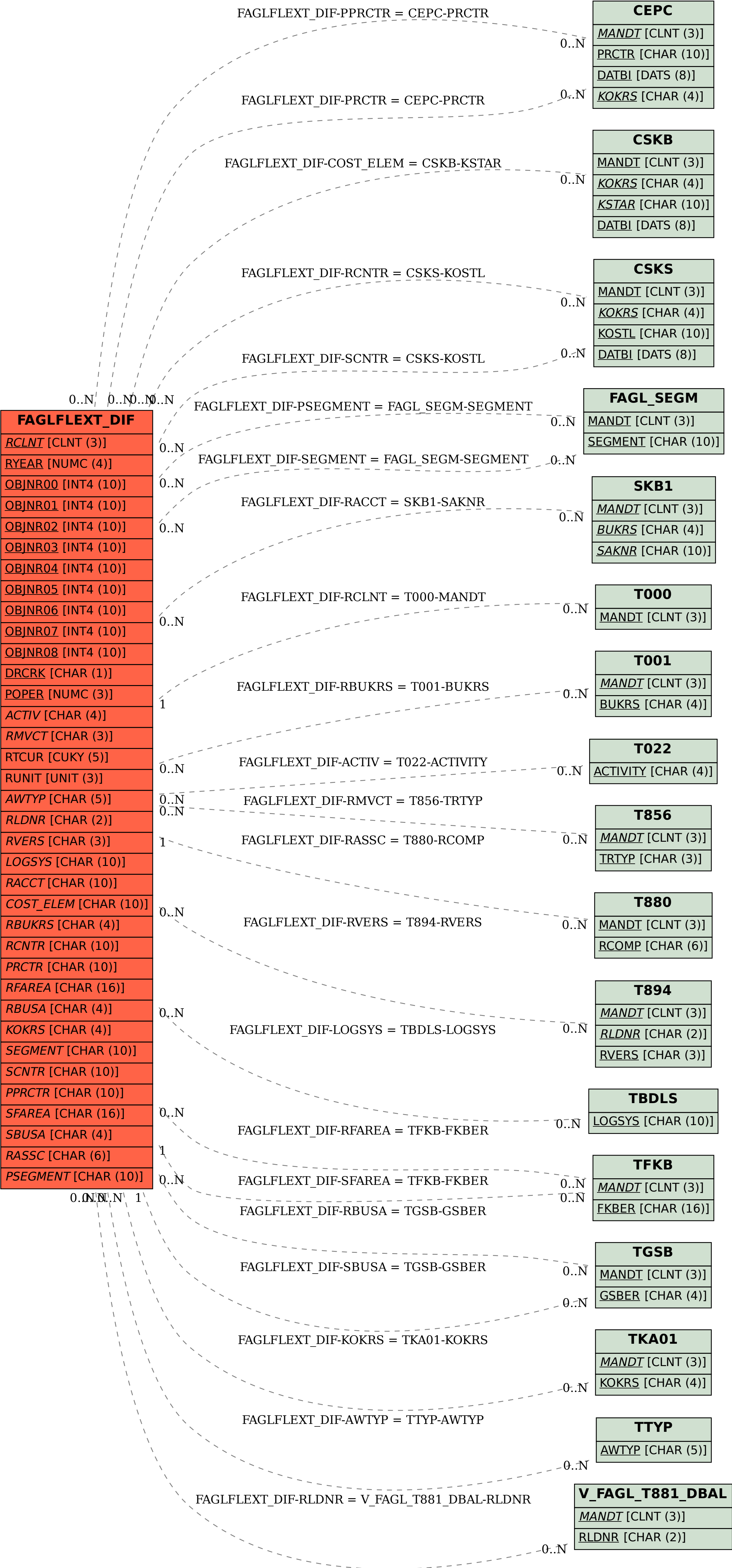
SAP ABAP table FAGLFLEXT_DIF {Delta Table: G/L Totals}
