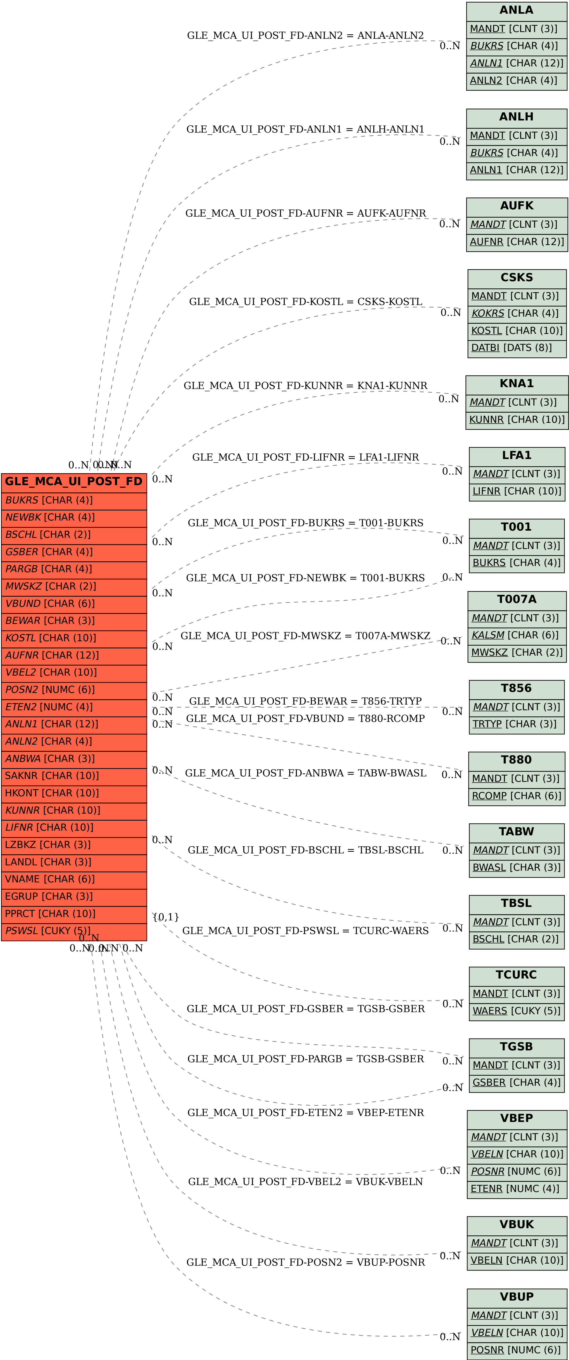
SAP ABAP table GLE_MCA_UI_POST_FD {General information of posting line items of screen}
