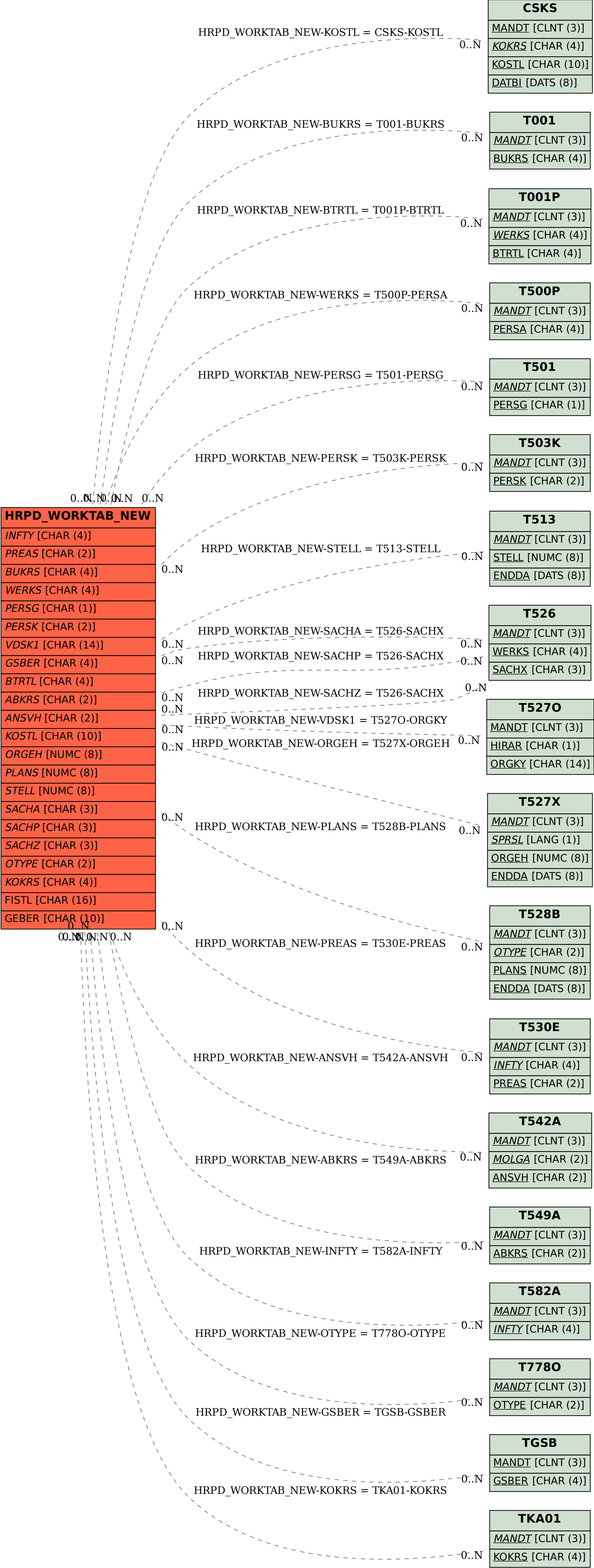
SAP ABAP table HRPD_WORKTAB_NEW {Structure for Work Table Integration PA - PD}
