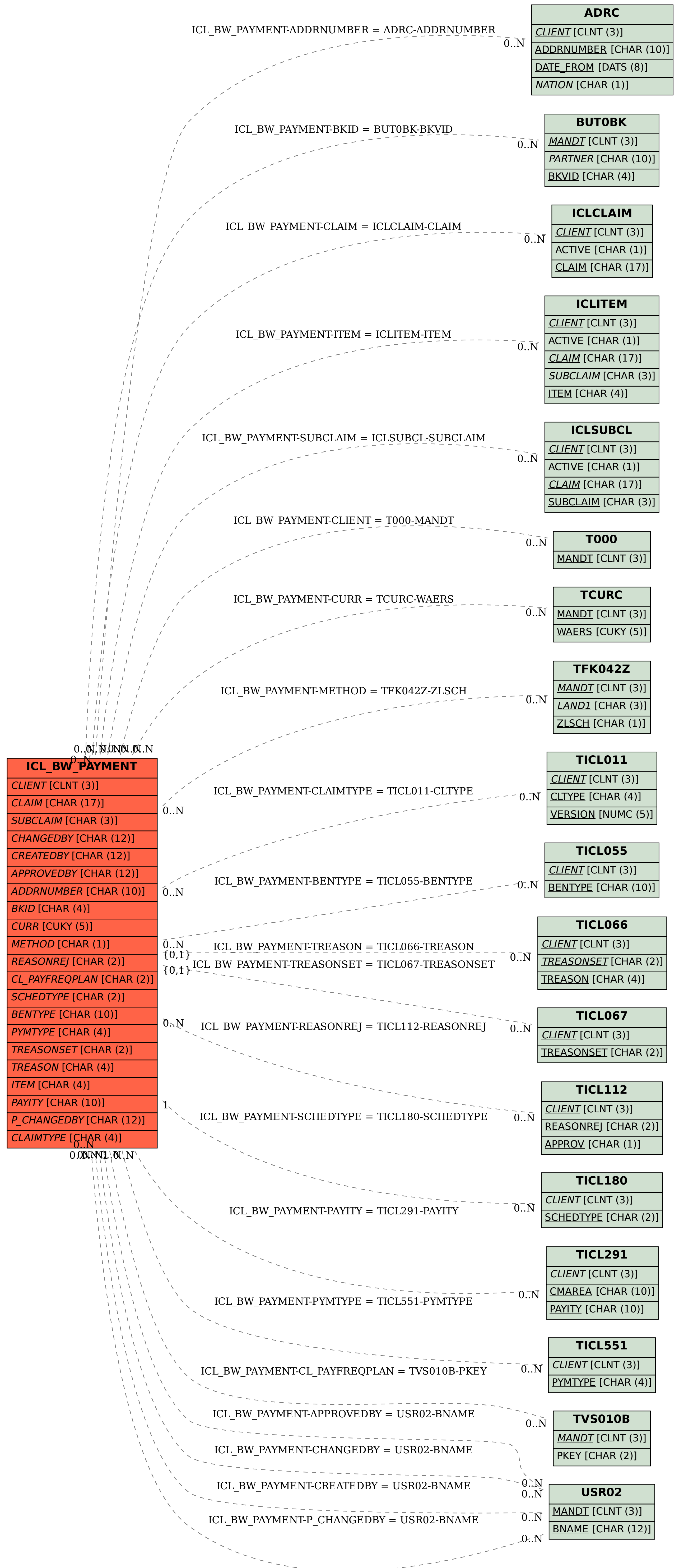
SAP ABAP table ICL_BW_PAYMENT {Extract Structure for Claim Payments (Header + Items)}
