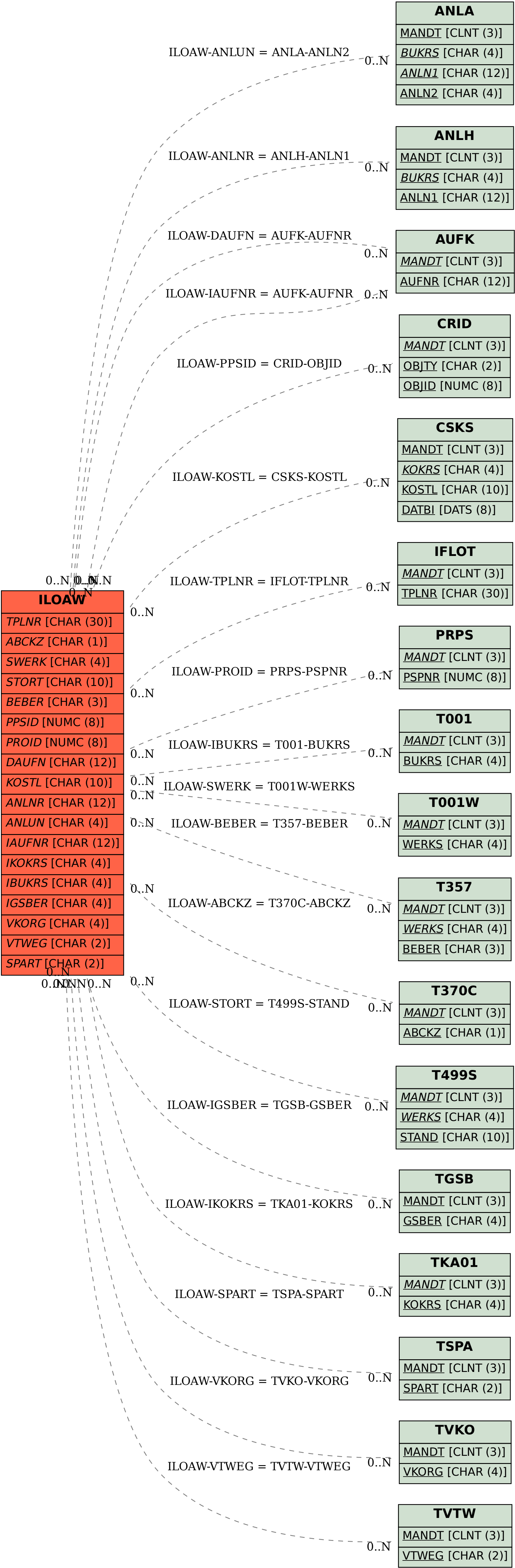
SAP ABAP table ILOAW {WORK STRUCTURE LOCATION AND ACCOUNT ASSIGNMENT DATA}
