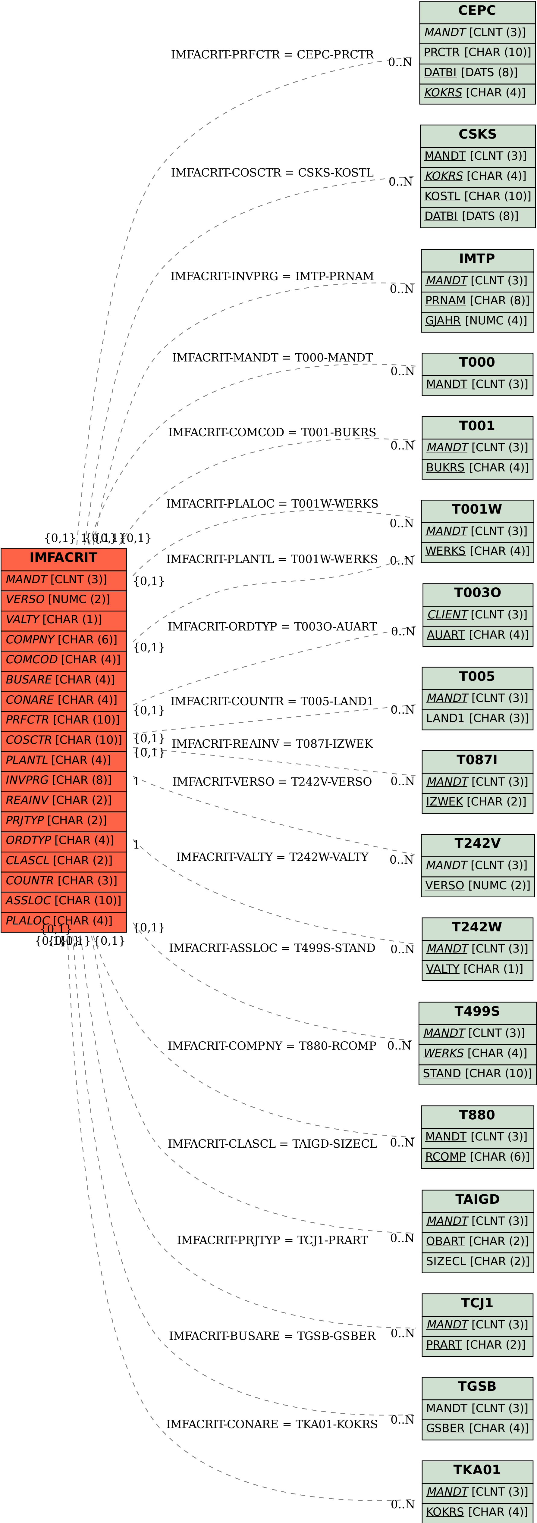
SAP ABAP table IMFACRIT {Characteristics for data transfer IM-FA/PS/CO-OPA to EIS}
