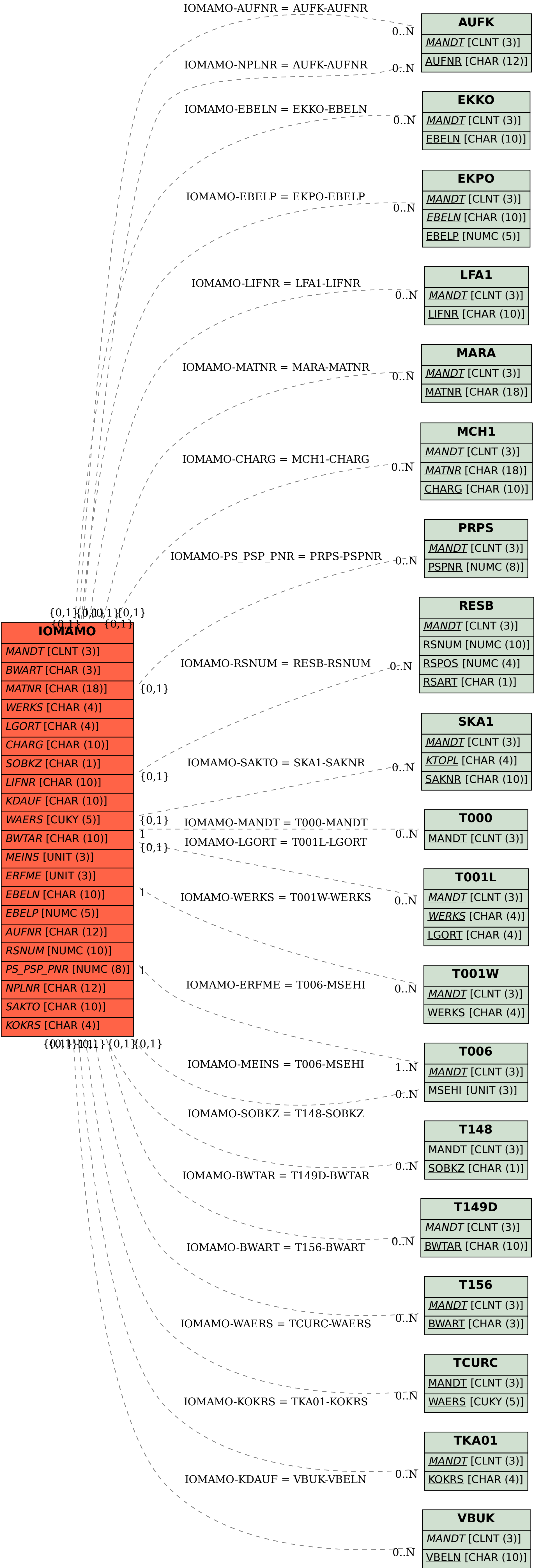
SAP ABAP table IOMAMO {Database structure for documentation goods movements}
