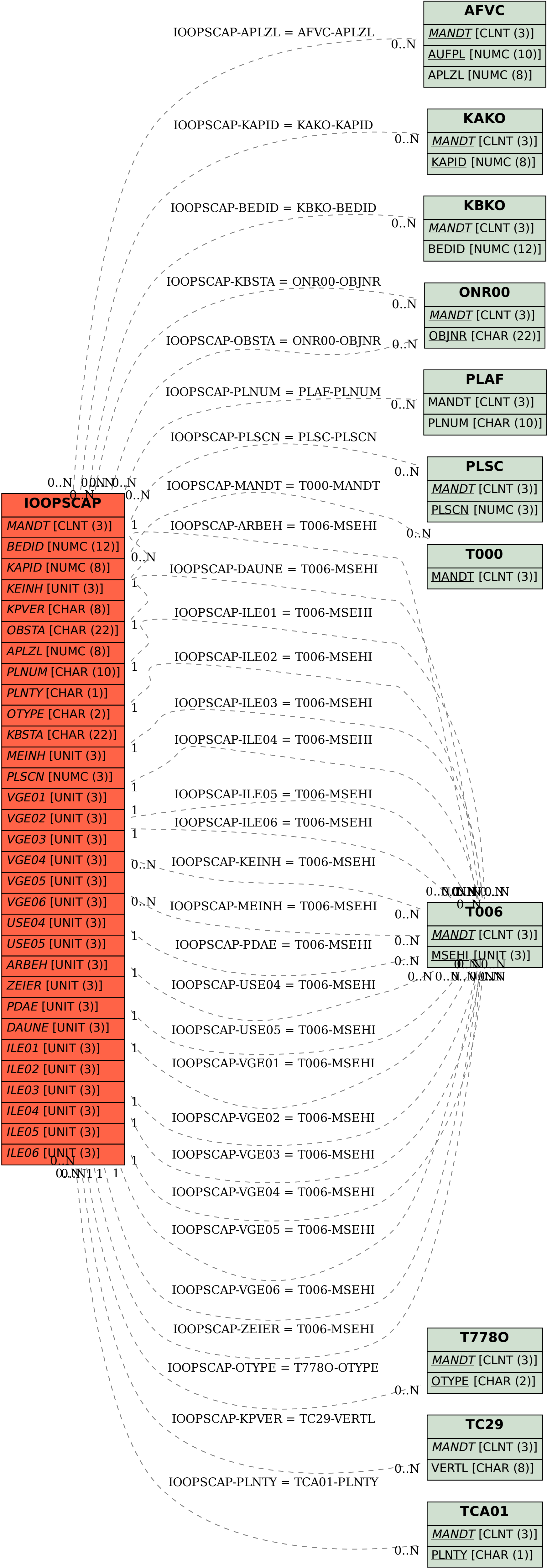
SAP ABAP table IOOPSCAP {Database structure individual capacities - order operations}
