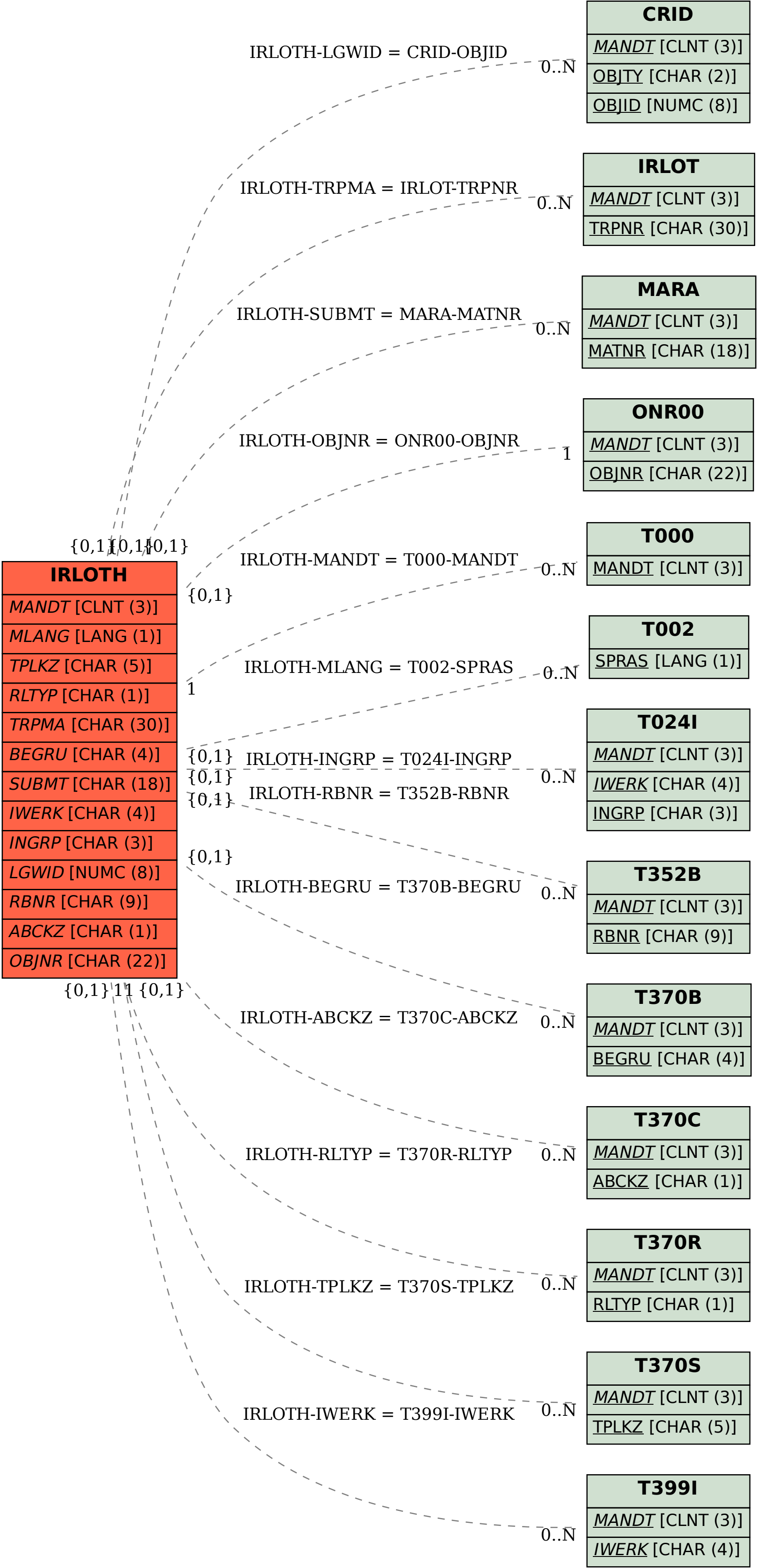
SAP ABAP table IRLOTH {Technical Reference Location (Table) With Hierarchy Level}
