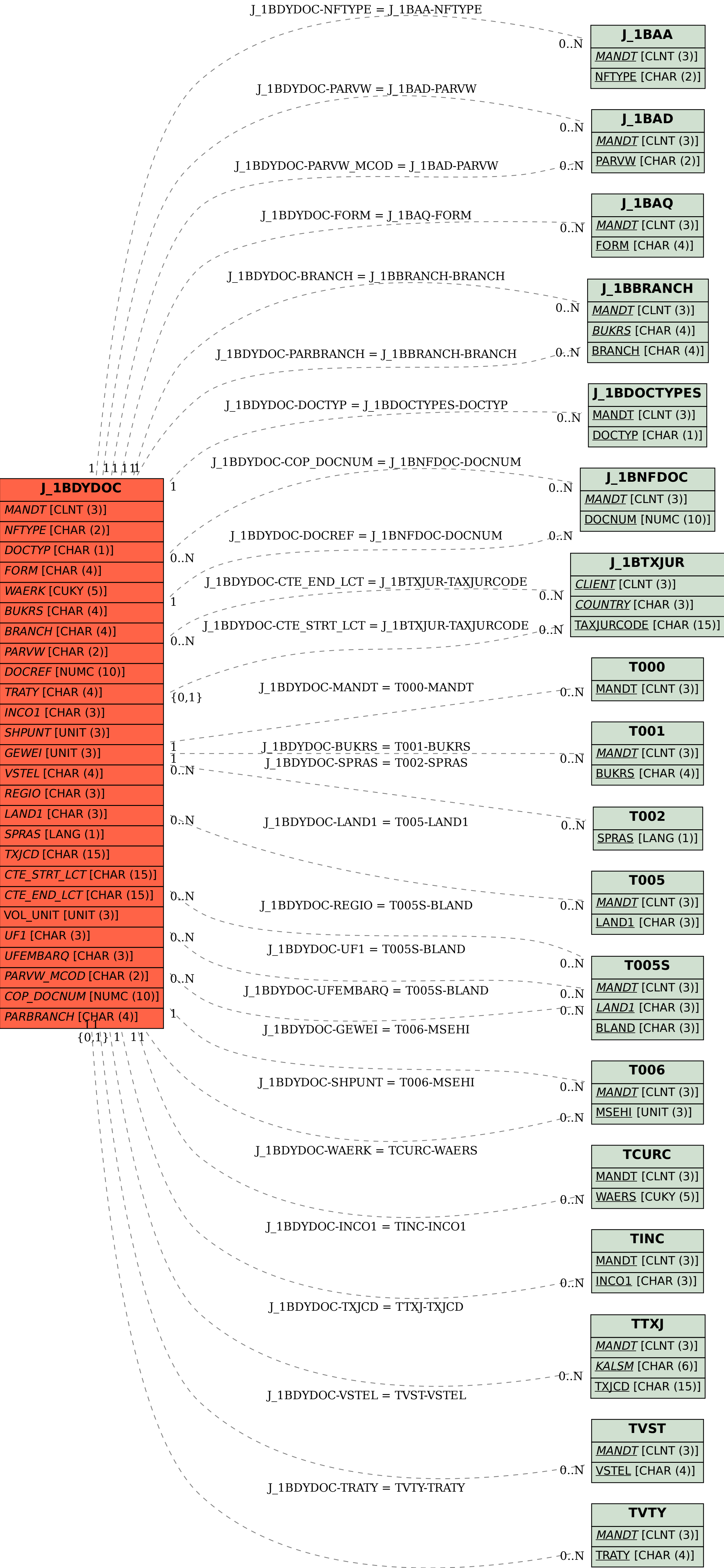
SAP ABAP table J_1BDYDOC {Dynpro fields for Nota Fiscal header (Edit function)}
