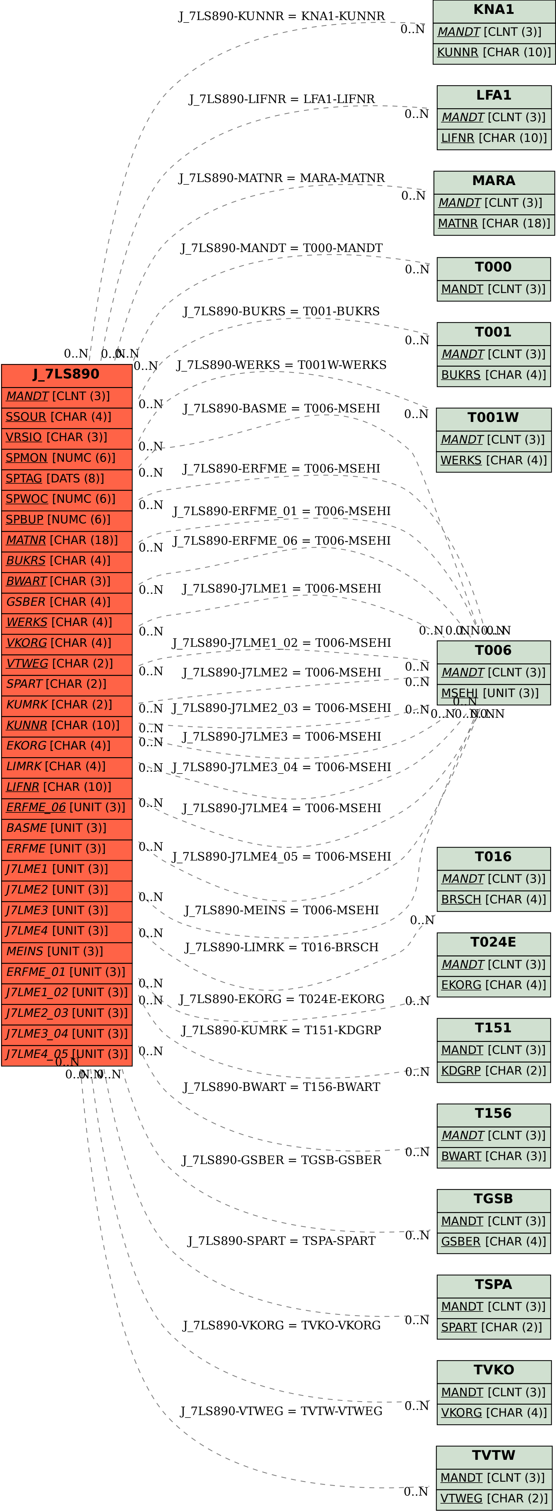
SAP ABAP table J_7LS890 {REA Reference for Info Structure Material Movements}
