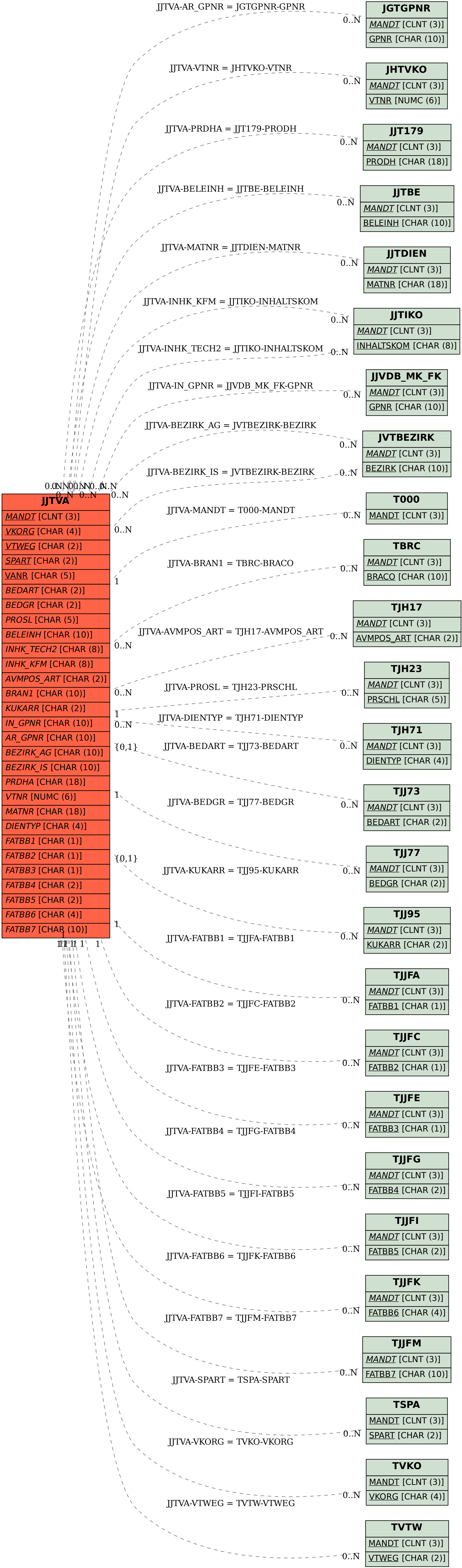
SAP ABAP table JJTVA {Incl/Exclusive Sales Agt Requirements for Entire Sales Area}
