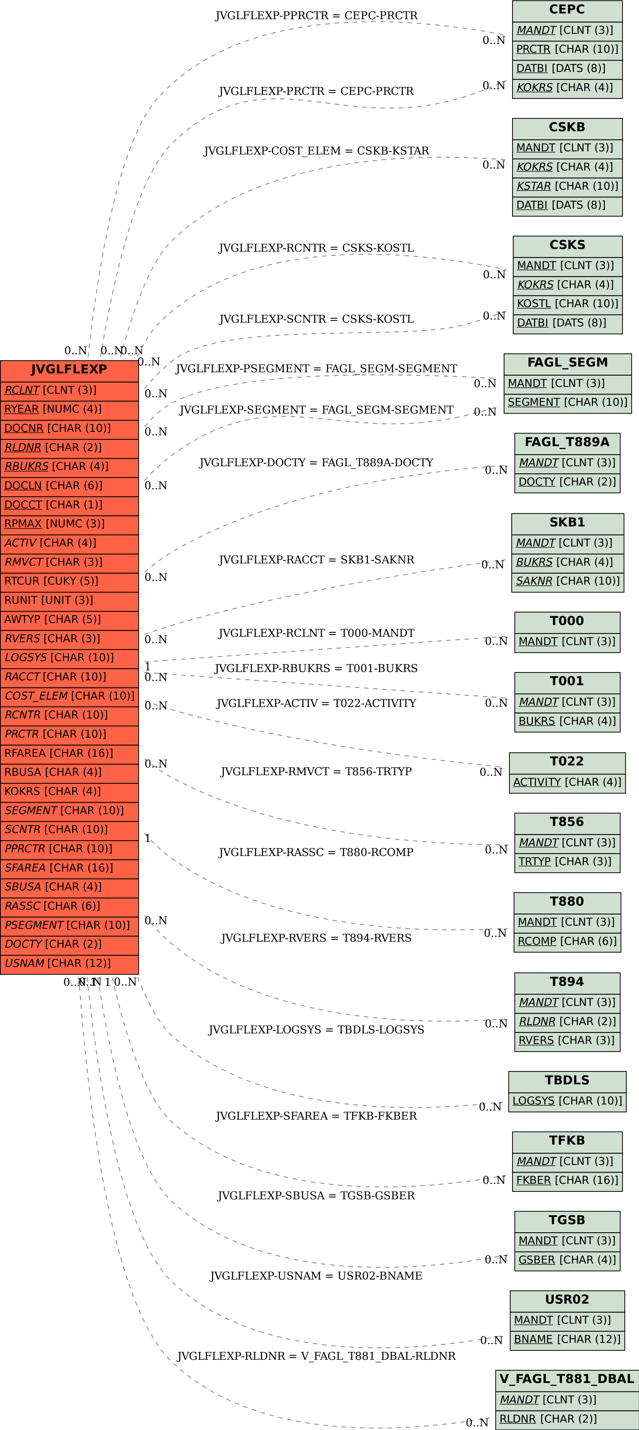
SAP ABAP table JVGLFLEXP {General Ledger: Plan Line Items}
