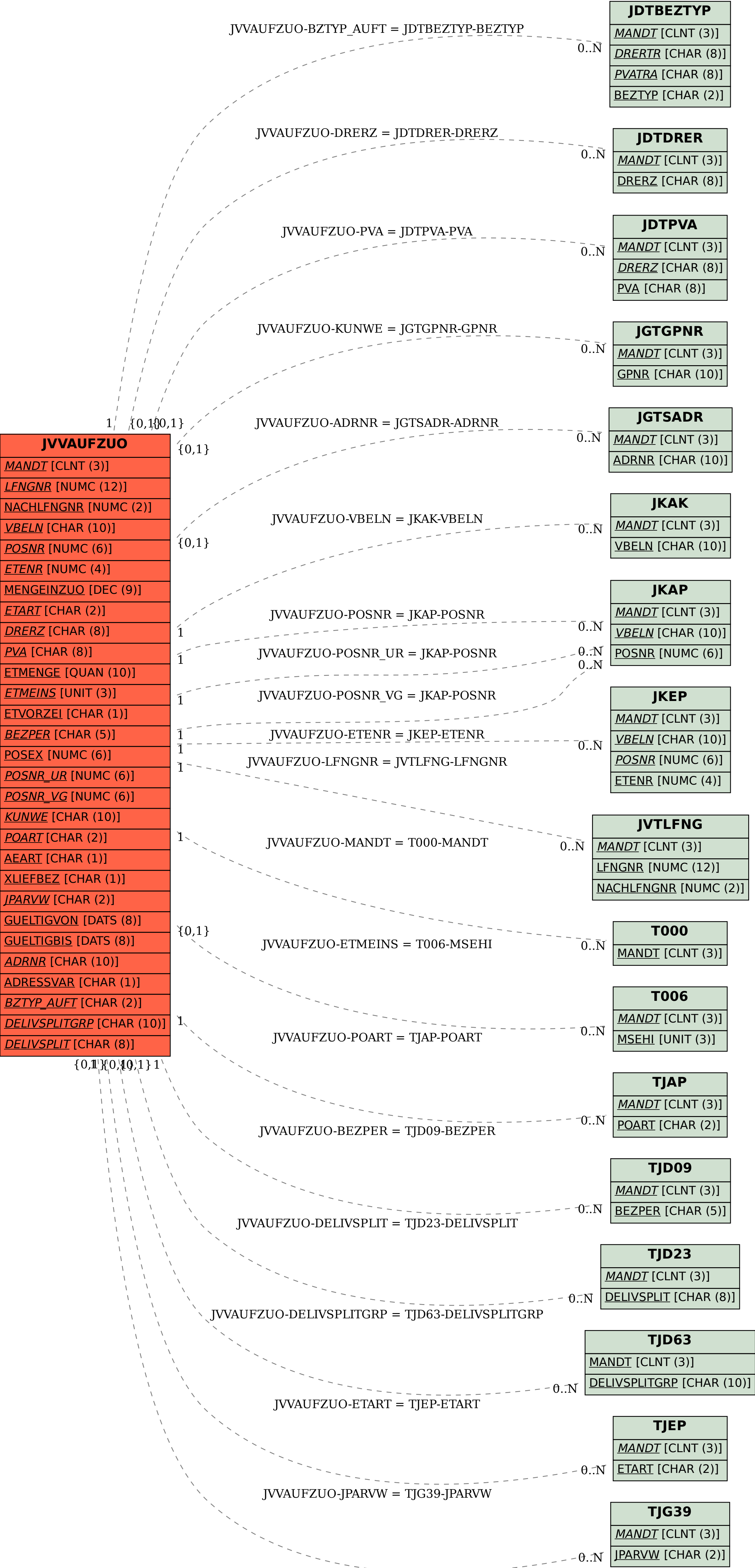
SAP ABAP table JVVAUFZUO {Generated Table for View}
