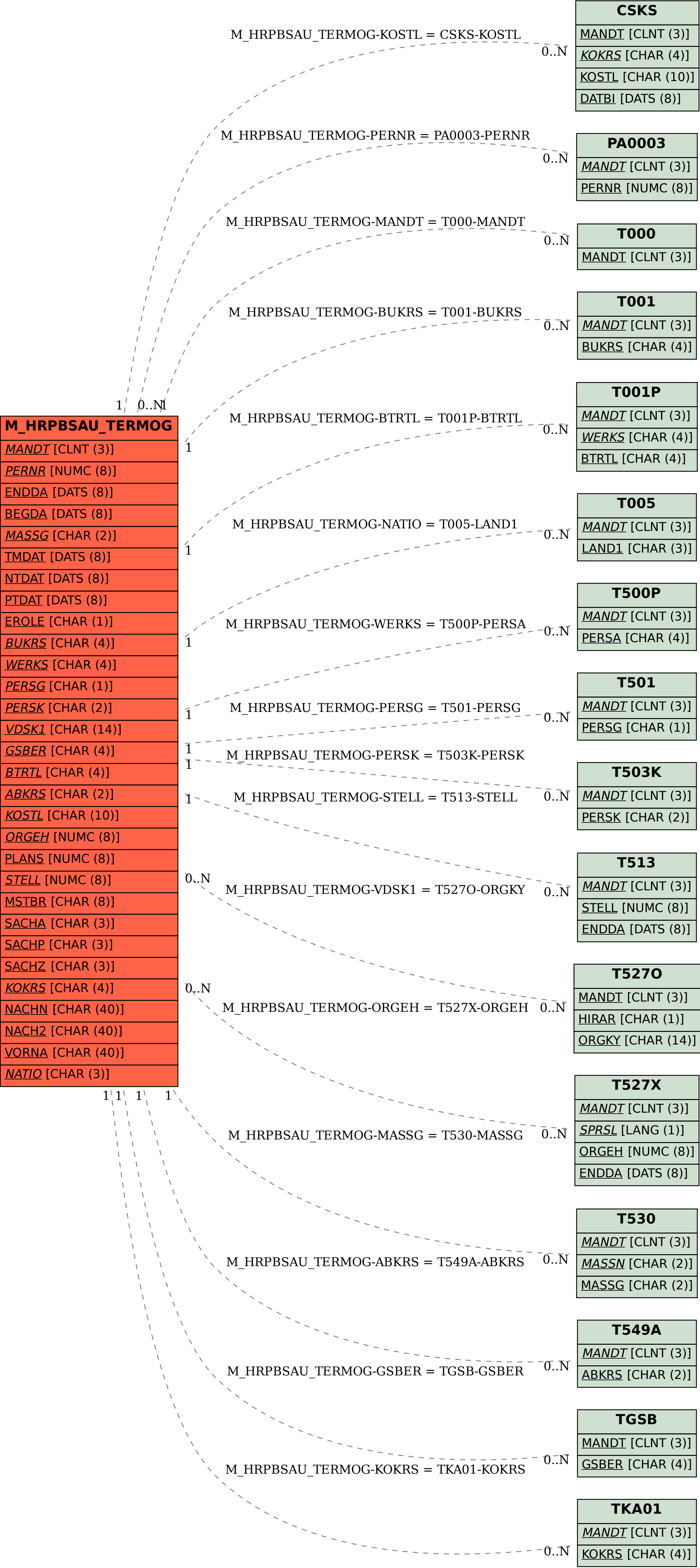
SAP ABAP table M_HRPBSAU_TERMOG {Generated Table for View}
