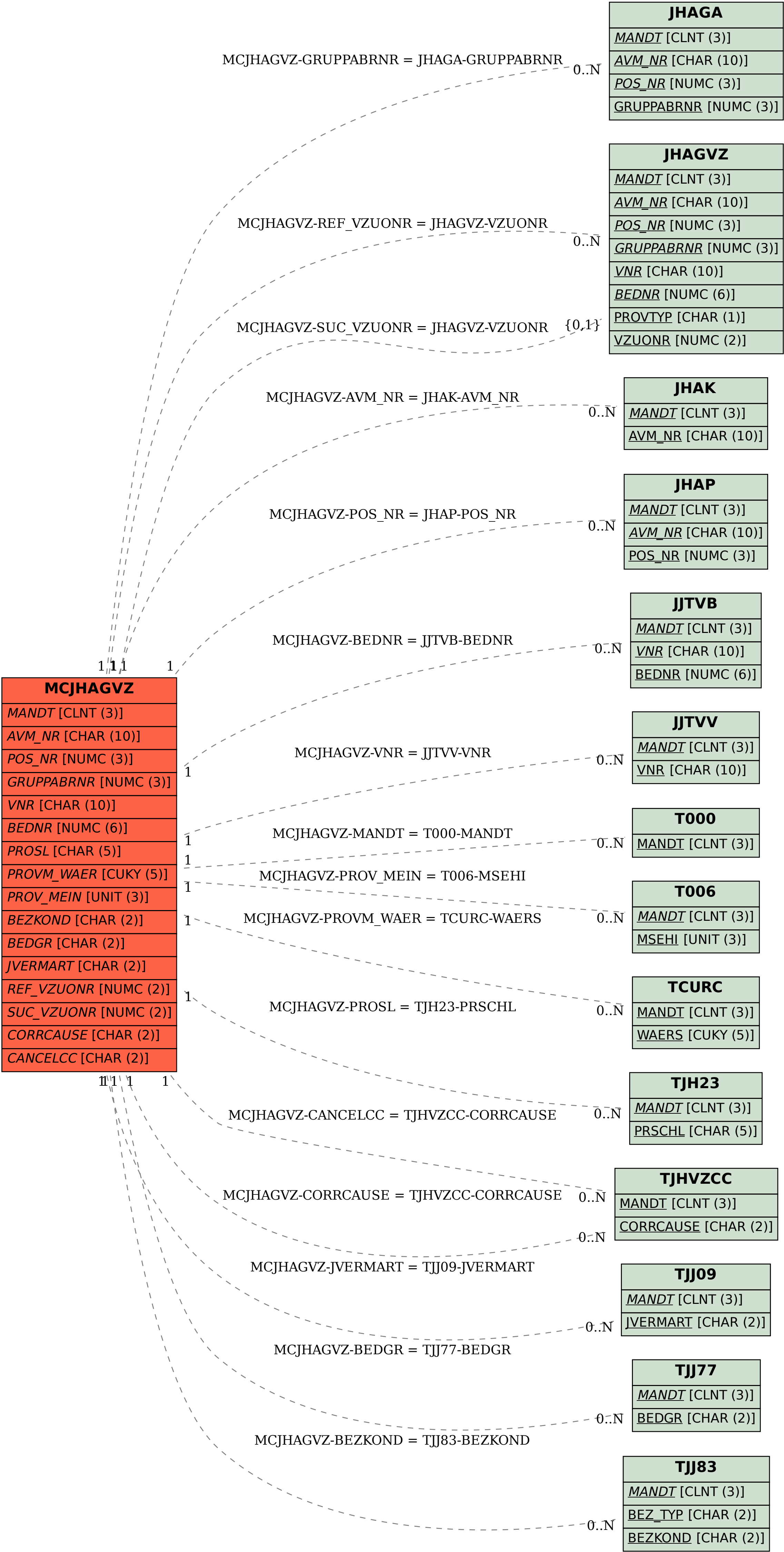
SAP ABAP table MCJHAGVZ {IS-PAM: LIS communication structure for agent assignment}
