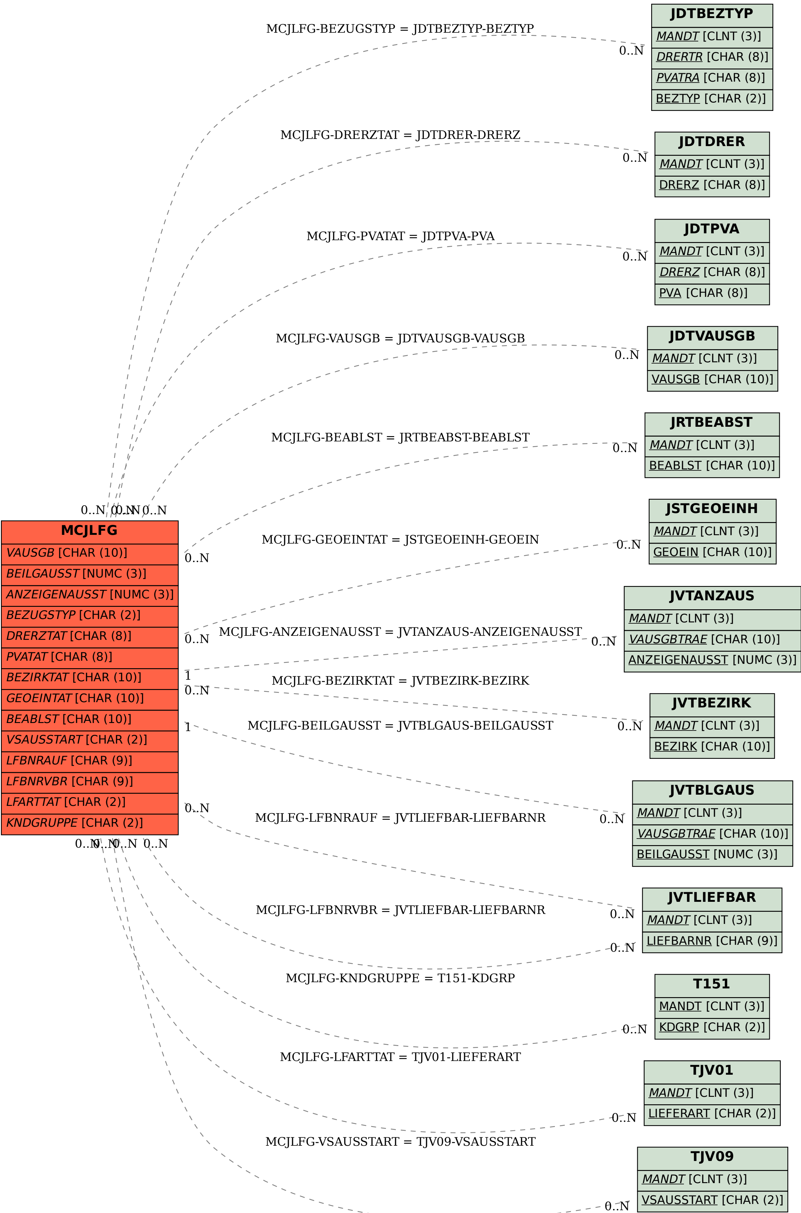
SAP ABAP table MCJLFG {IS-M/SD: Delivery Header Data, LIS Communication Structure}
