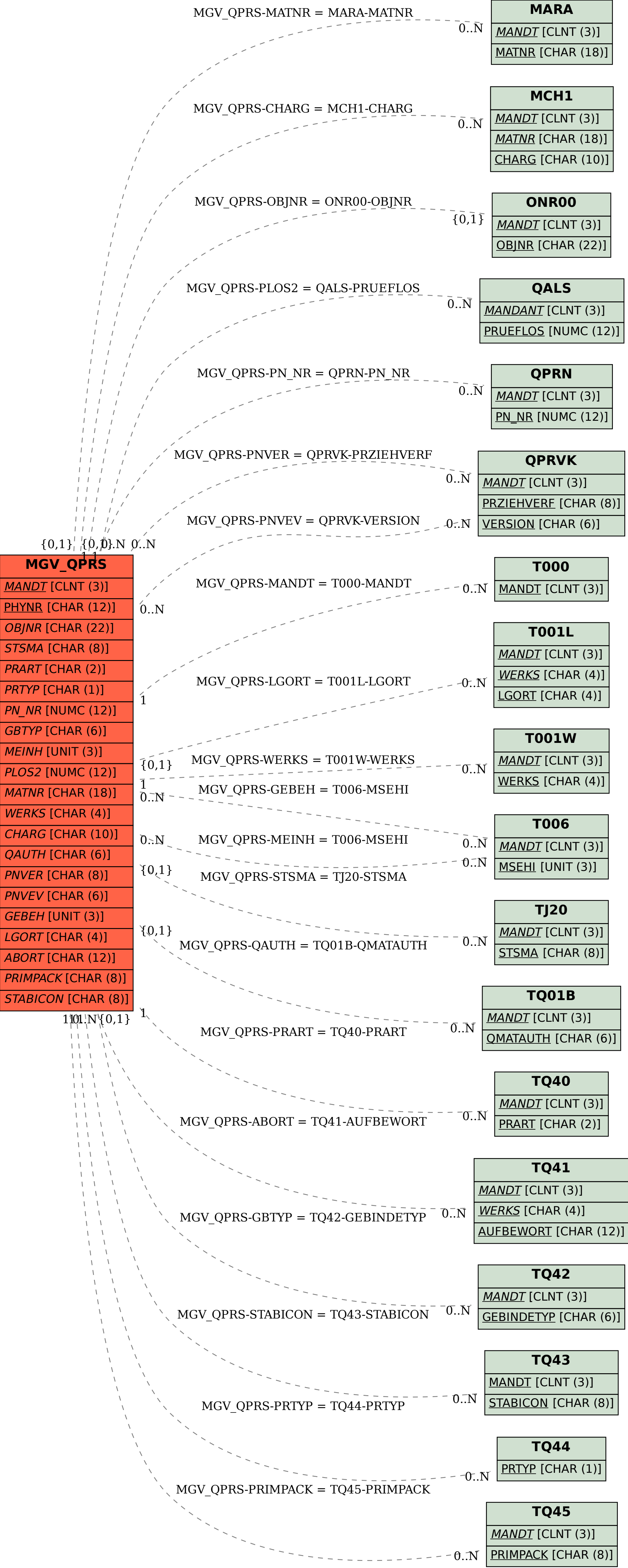
SAP ABAP table MGV_QPRS {Generated Table for View MGV_QPRS}
