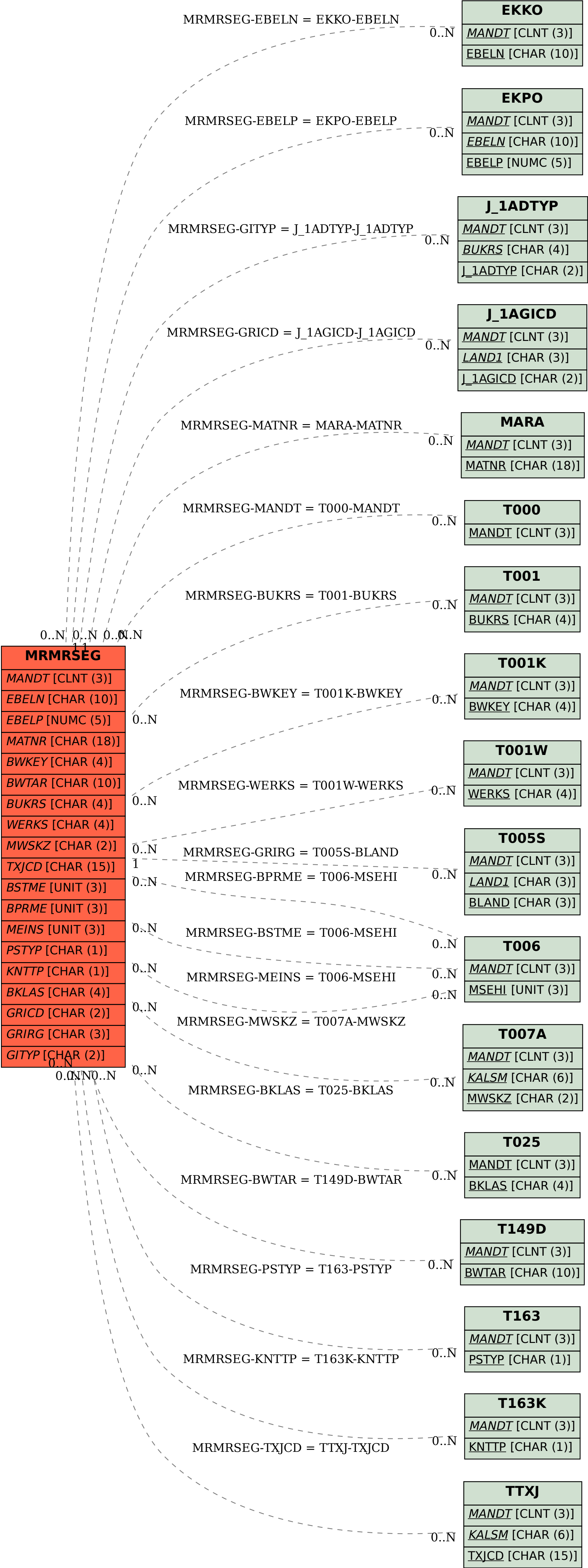
SAP ABAP table MRMRSEG {Change document structure; generated by RSSCD000}
