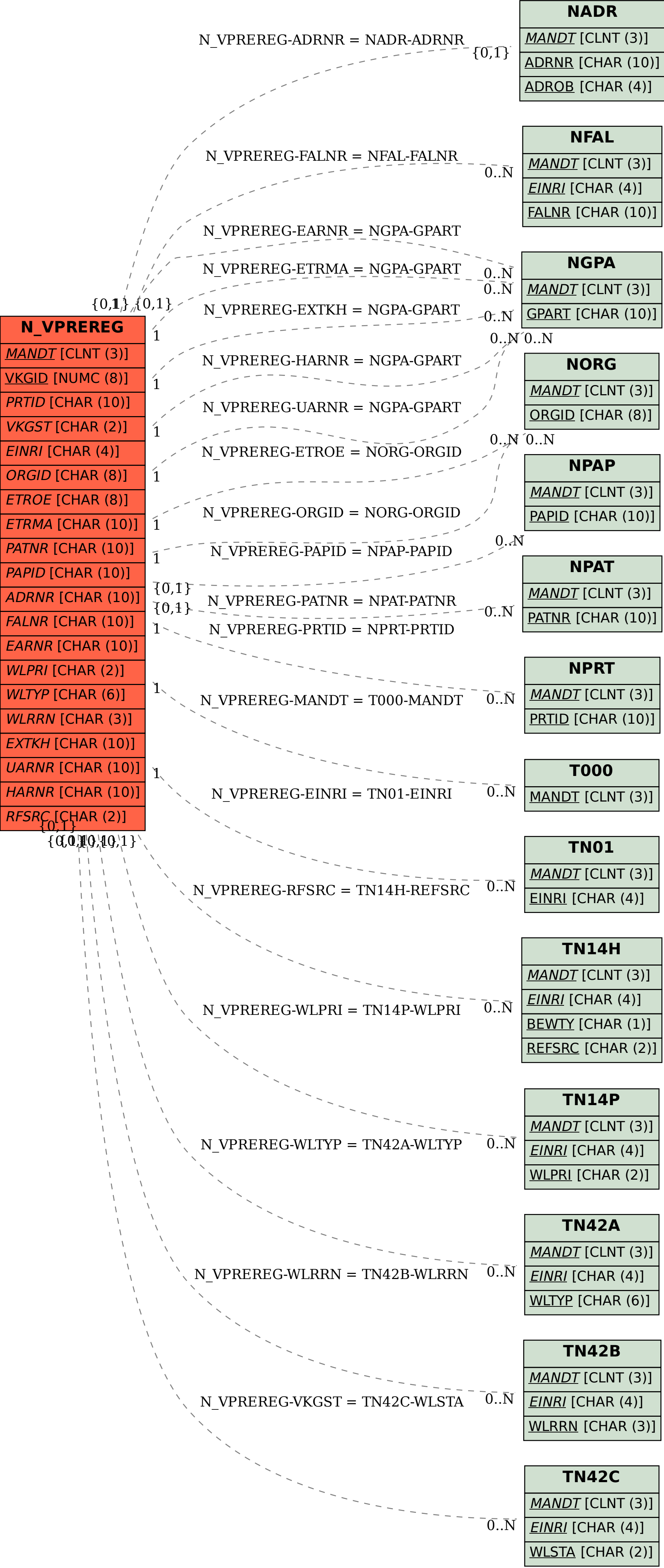
SAP ABAP table N_VPREREG {Generated Table for View}
