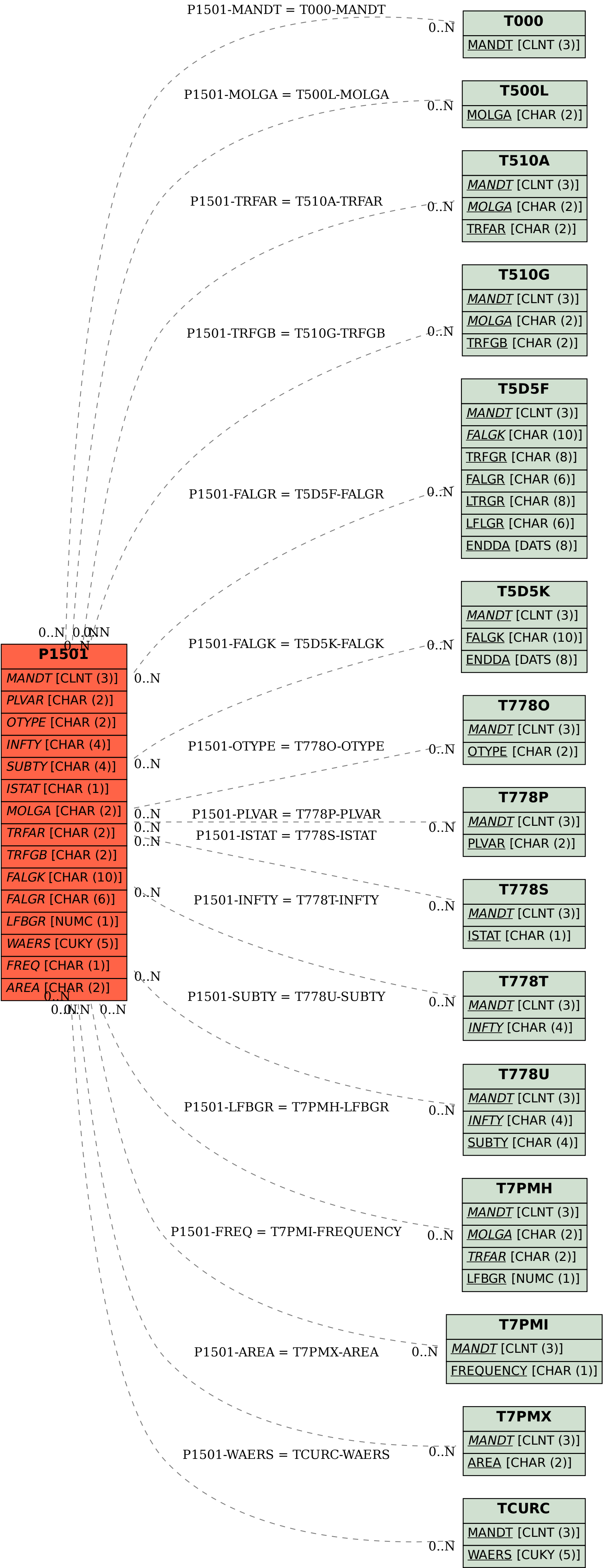
SAP ABAP table P1501 {Infotype 1501: HR-FPM Valuation (PSG Pay Scales)}
