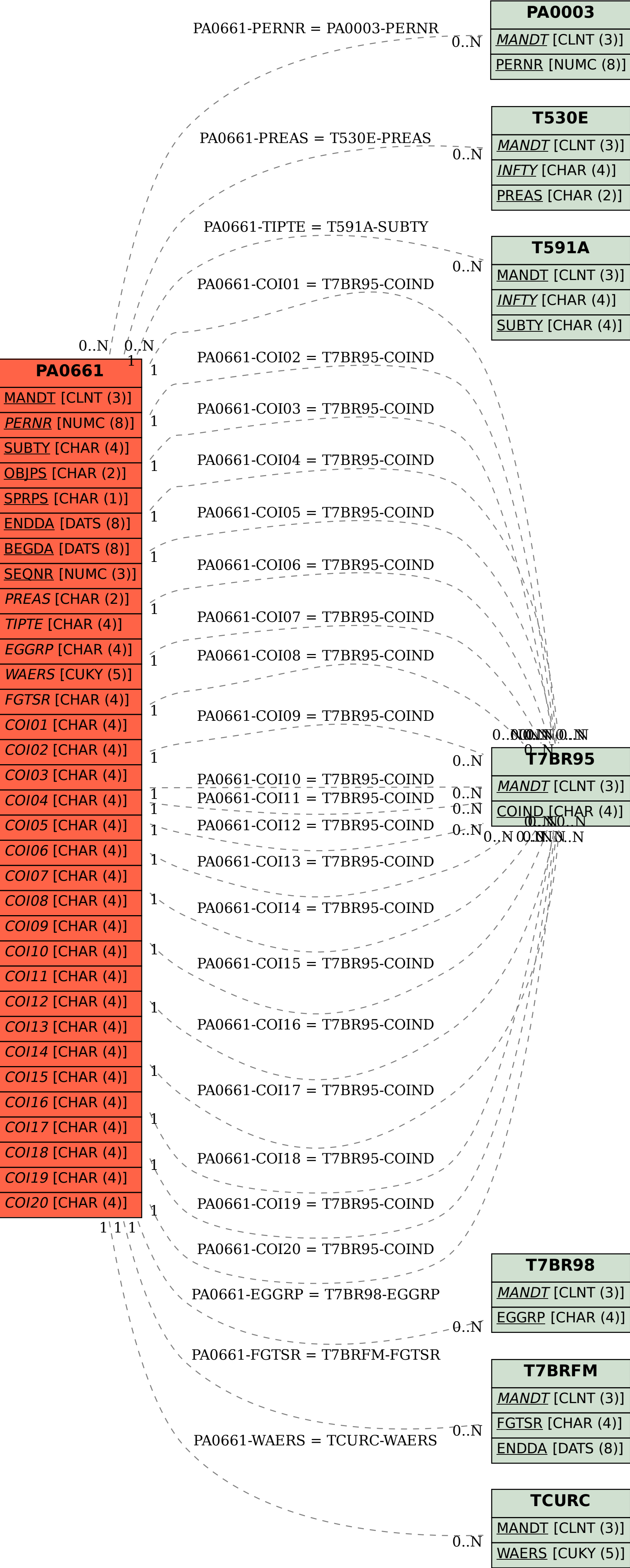
SAP ABAP table PA0661 {Termination: general data}
