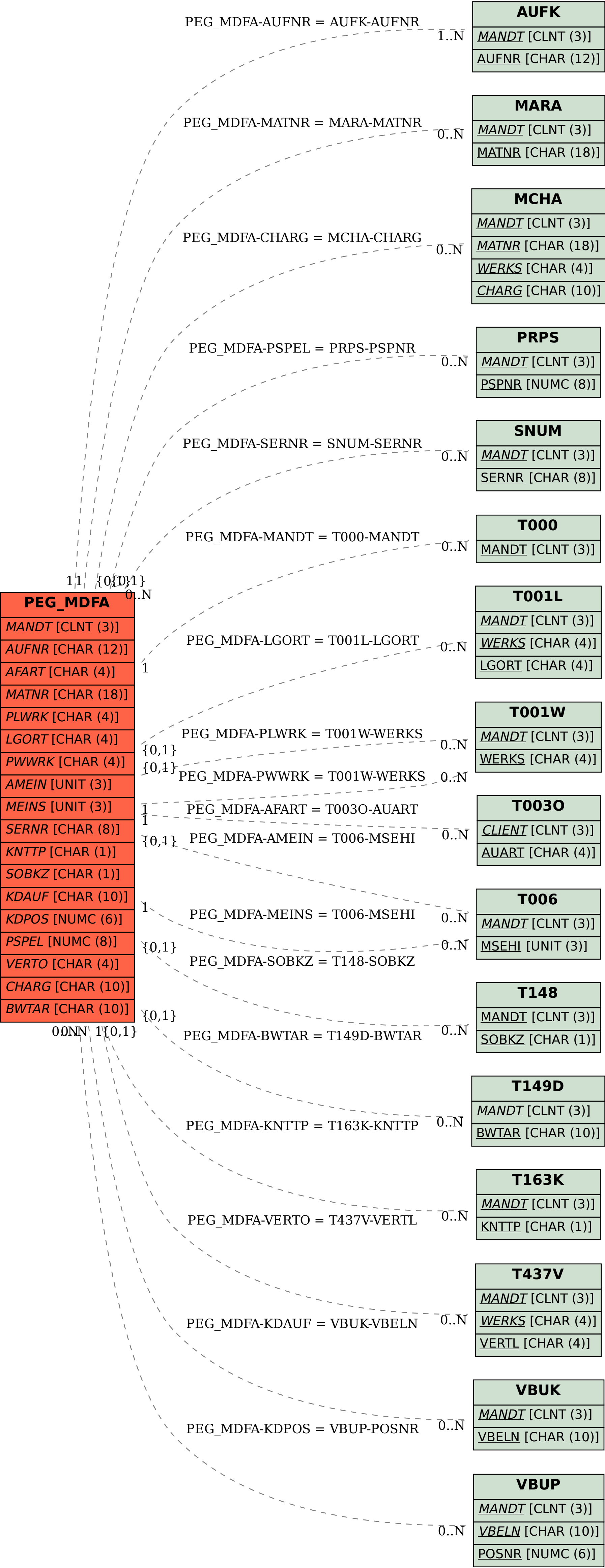
SAP ABAP table PEG_MDFA {Pegging: Production orders}
