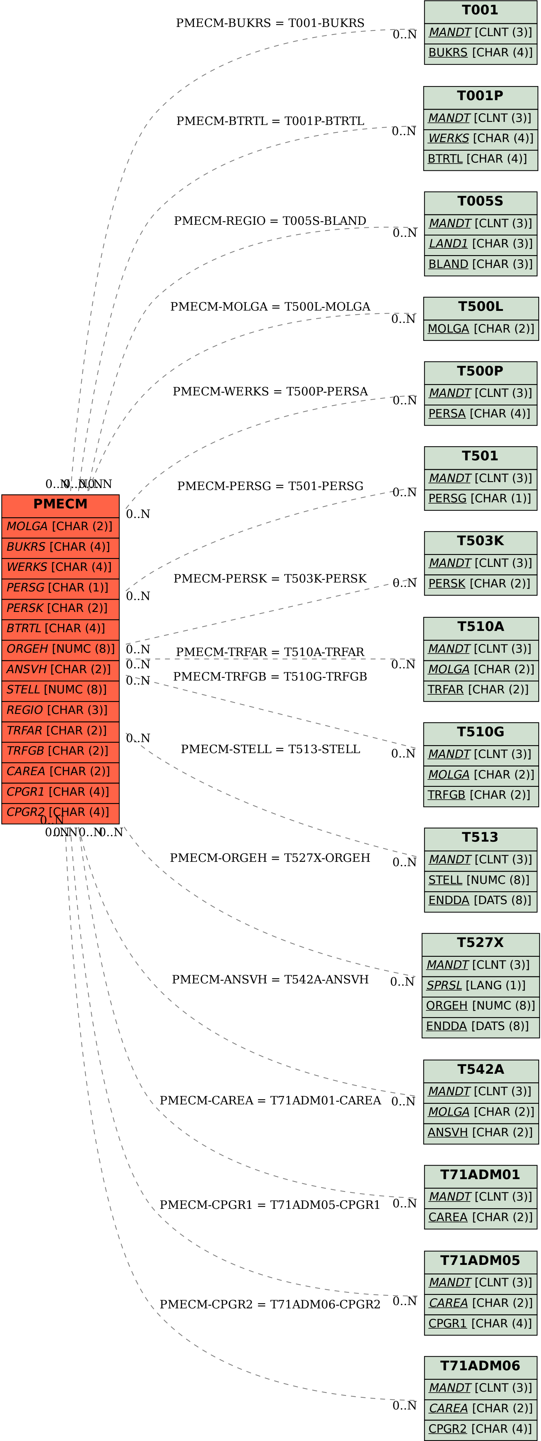
SAP ABAP table PMECM {Feature Decision Field Structure for Compensation Management}
