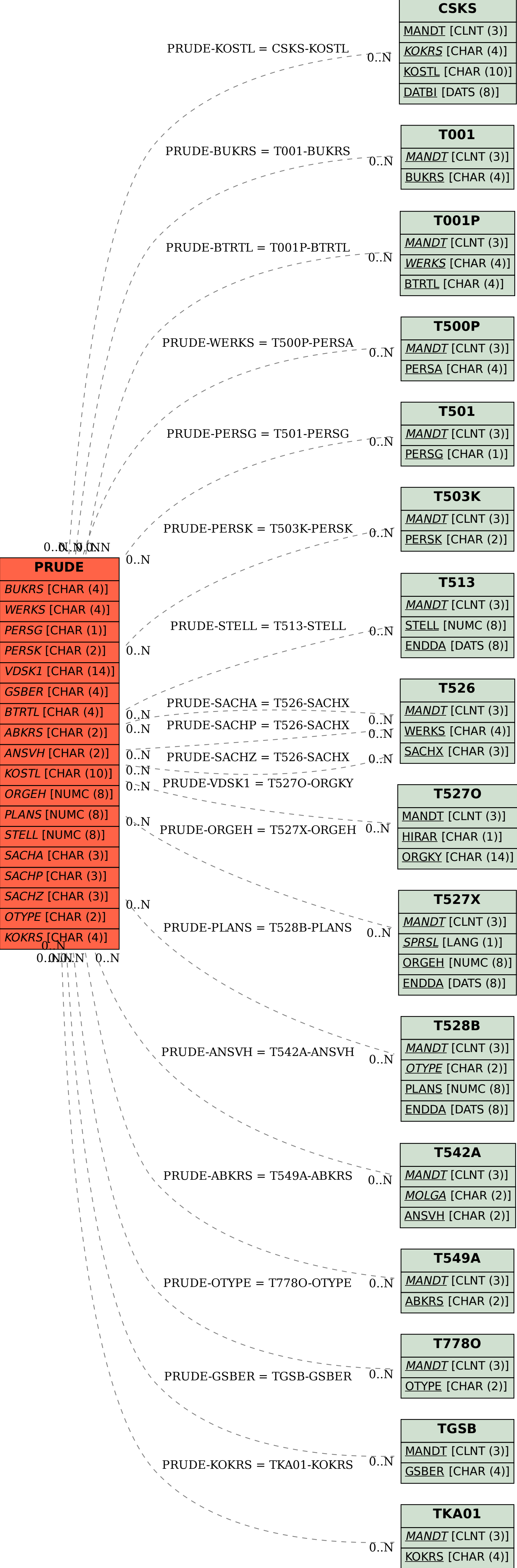
SAP ABAP table PRUDE {Structure for feature MMDAT}
