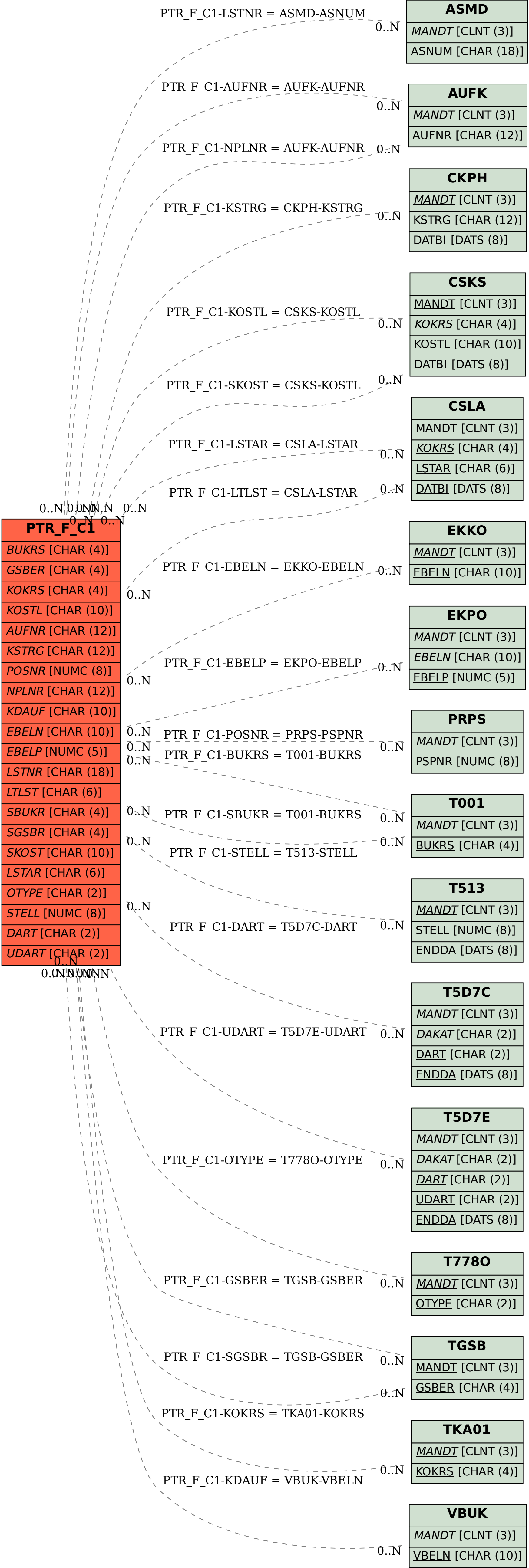
SAP ABAP table PTR_F_C1 {Row Type: C1 Time Statement Form}
