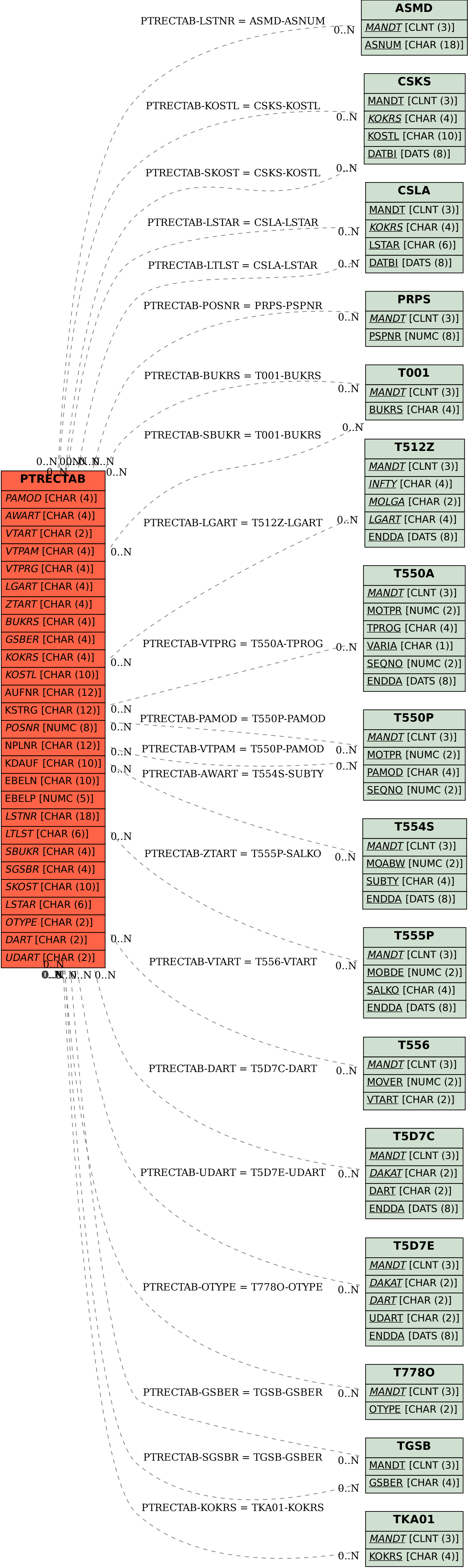
SAP ABAP table PTRECTAB {Line for Time Recording for Multiple Persons and Infotypes}
