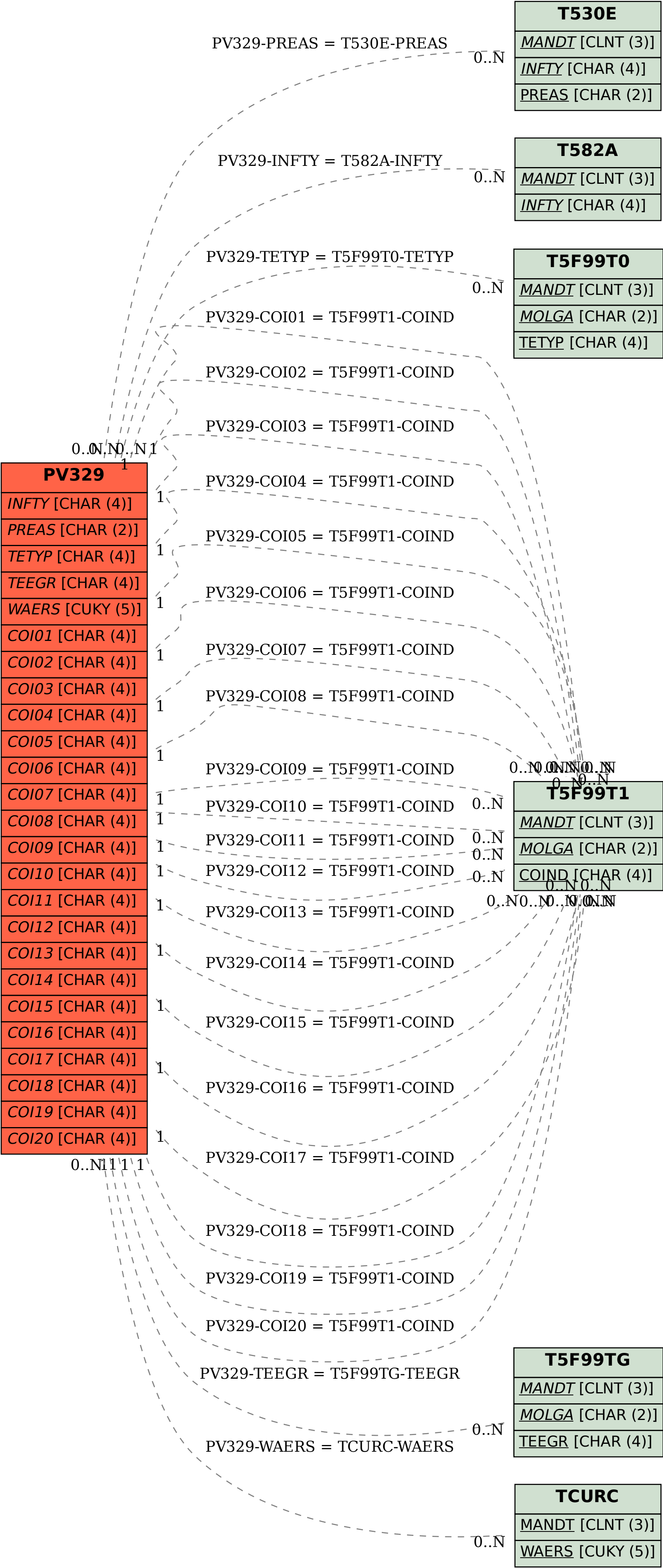
SAP ABAP table PV329 {Basic rec. of view 3298 (global view 0713)}
