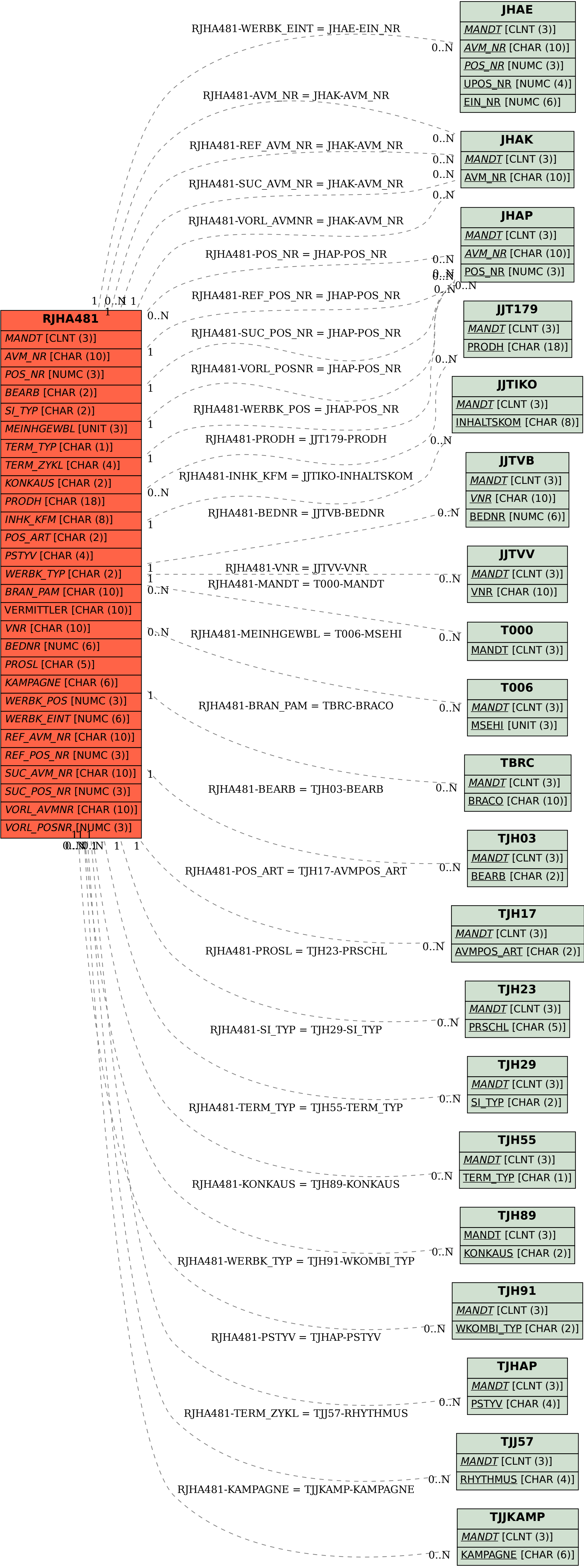
SAP ABAP table RJHA481 {IS-M/AM: Screen Structure for Ad Insert Item List}
