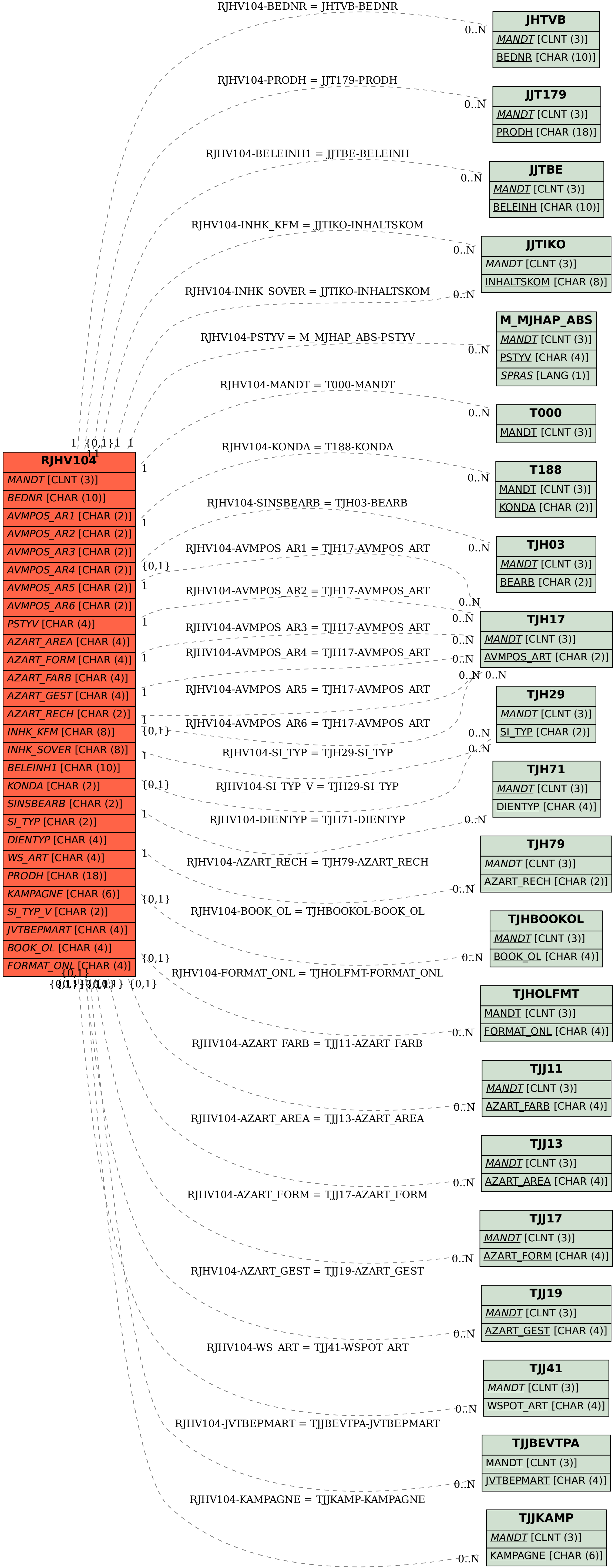
SAP ABAP table RJHV104 {IS-PAM: Int. table for maintaining conditions, screen 400}
